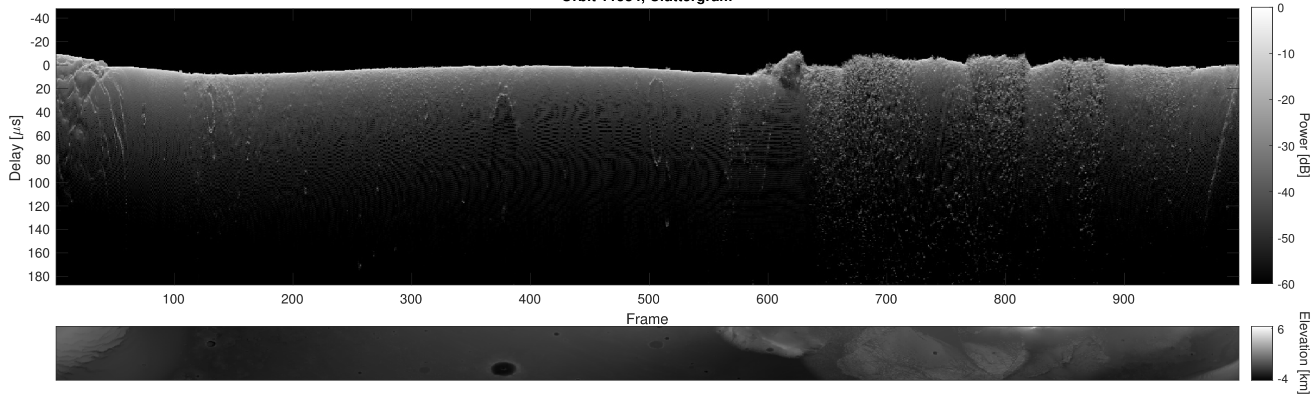
Orbit 11584, Cluttergram
