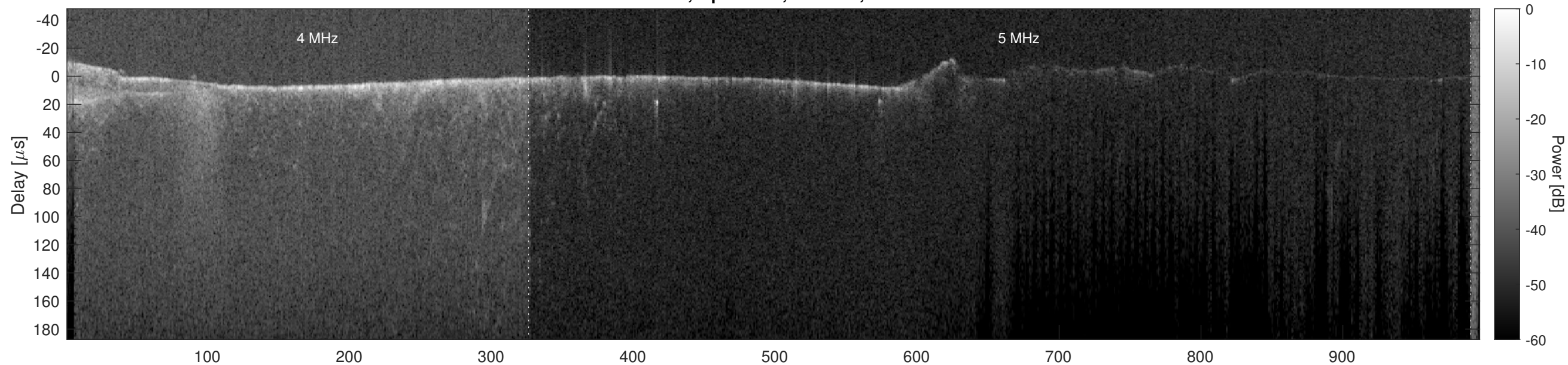
Orbit 11584, Optimized, Window, Channel 2
