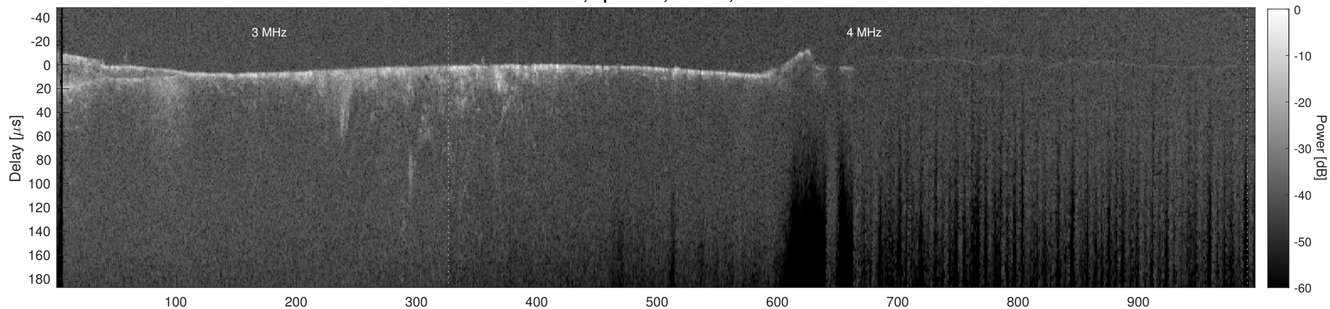
Orbit 11584, Cluttergram
