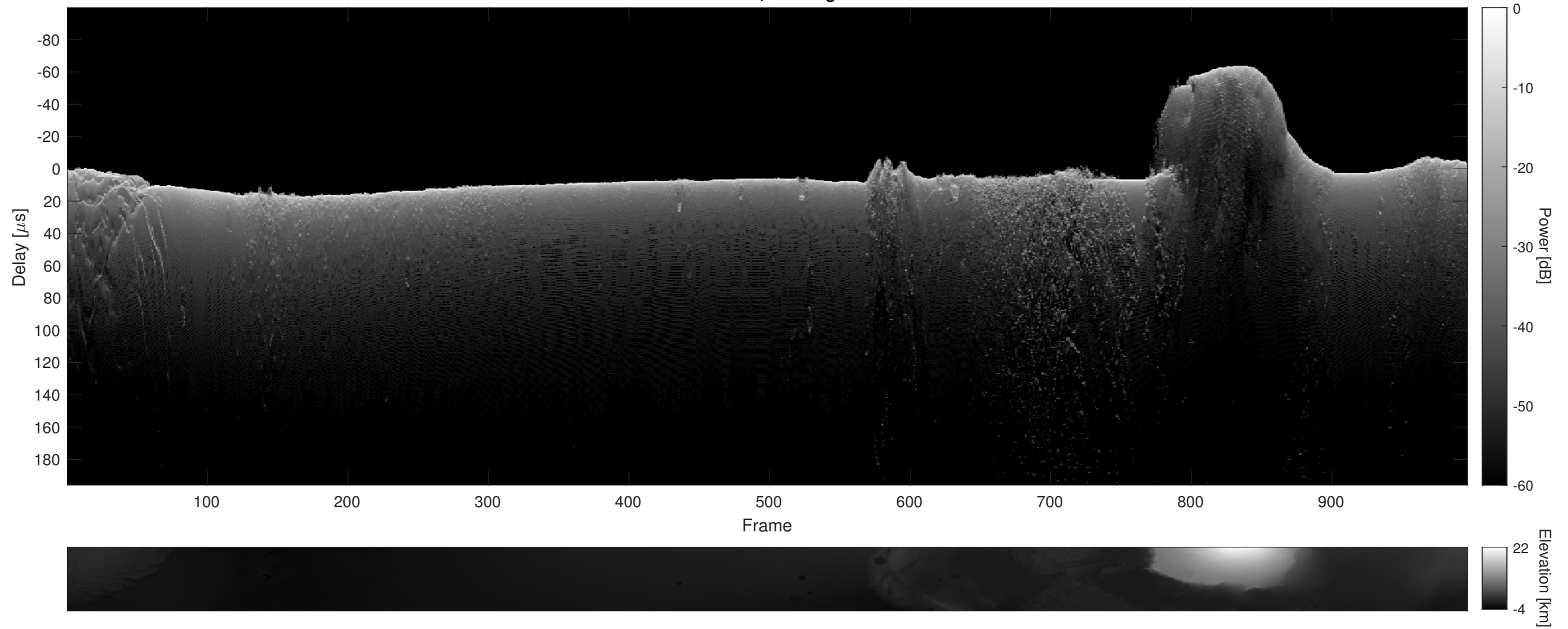
Orbit 11591, Cluttergram
