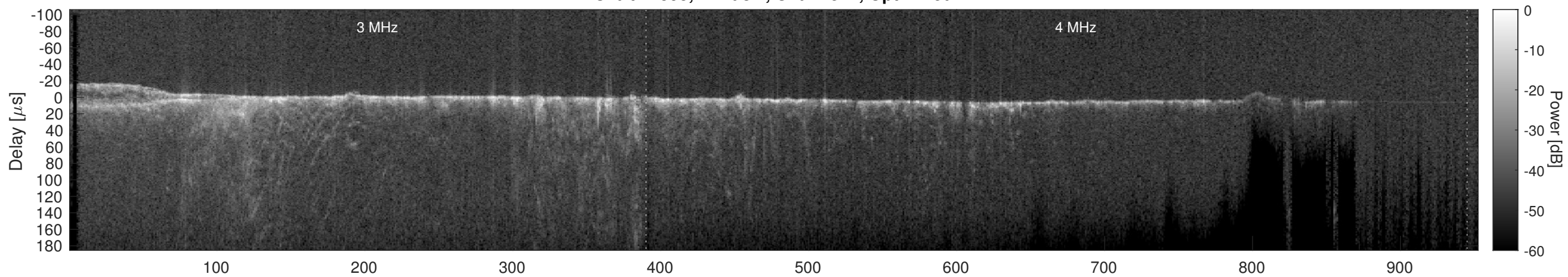
Orbit 11595, Cluttergram
