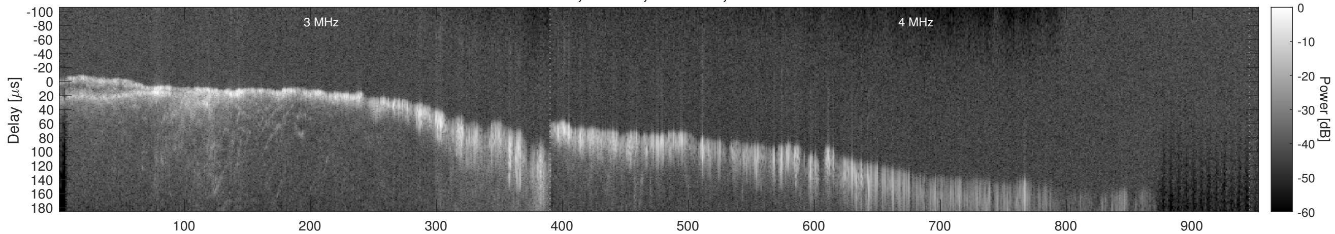
Orbit 11595, Window, Channel 2, Chapman
