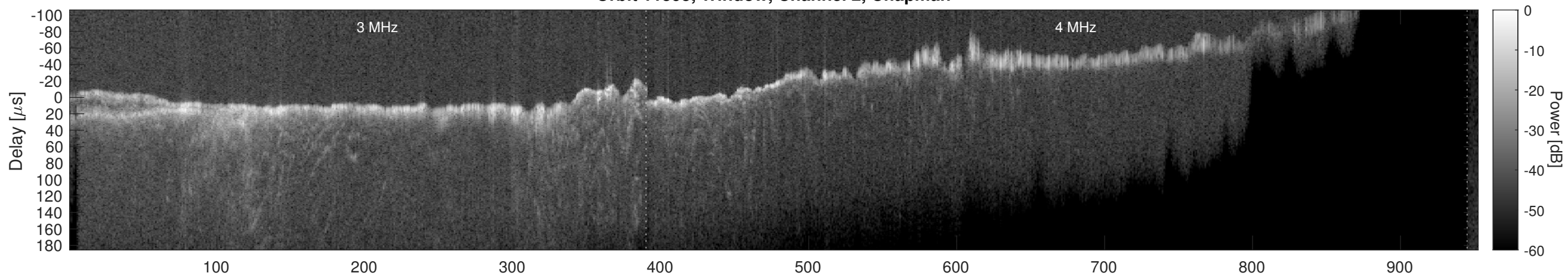
Orbit 11595, Window, Channel 2, Optimized
