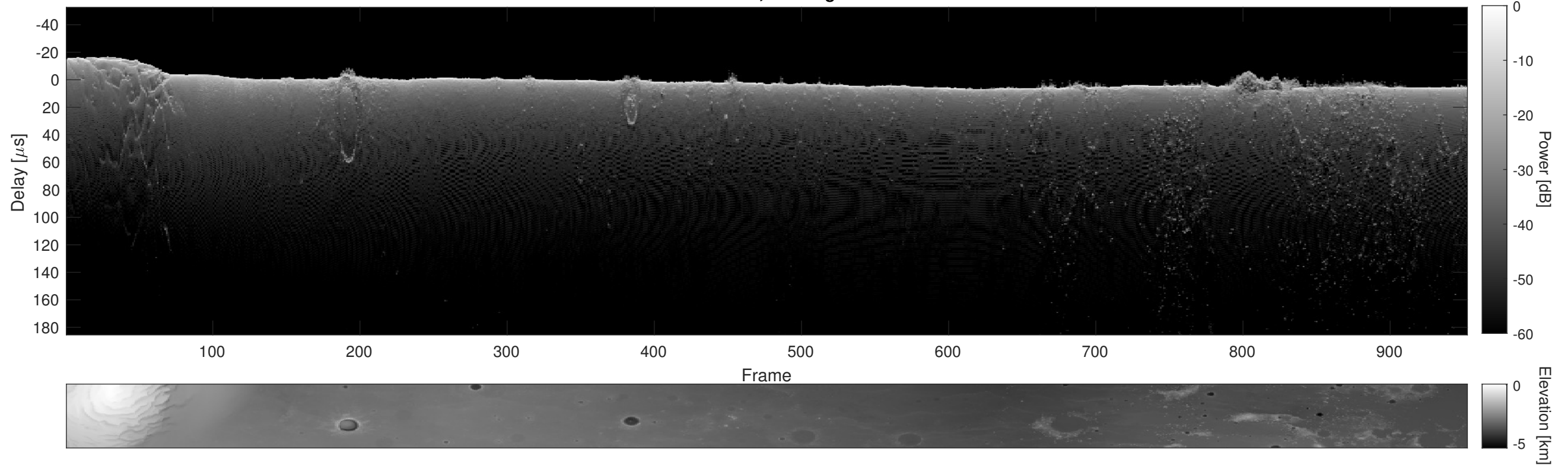
Orbit 11595, Cluttergram
