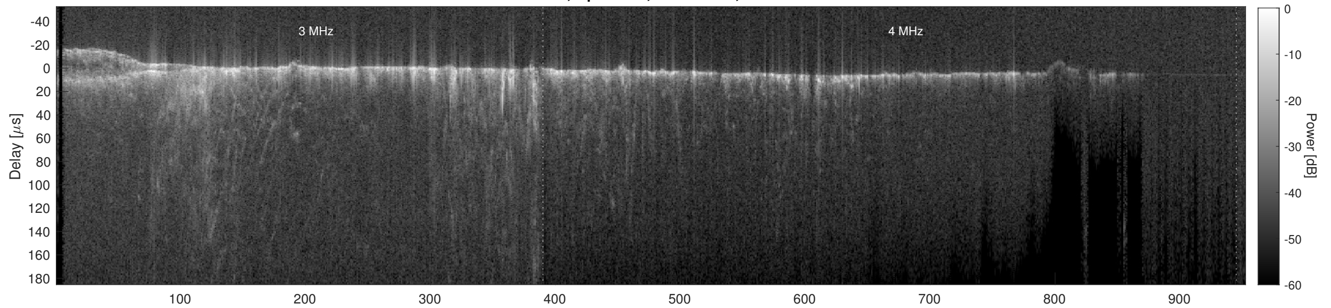
Orbit 11595, Cluttergram
