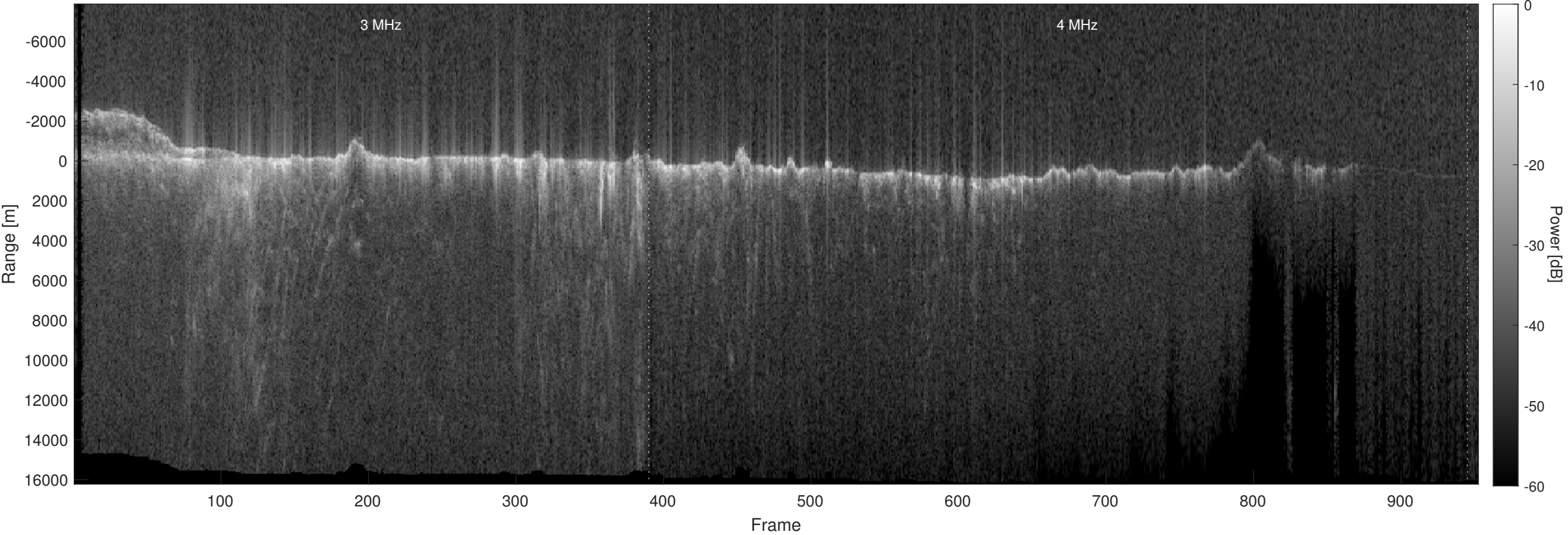
Orbit 11595, Optimized, No Window, Depth-Corrected, Channel 2
