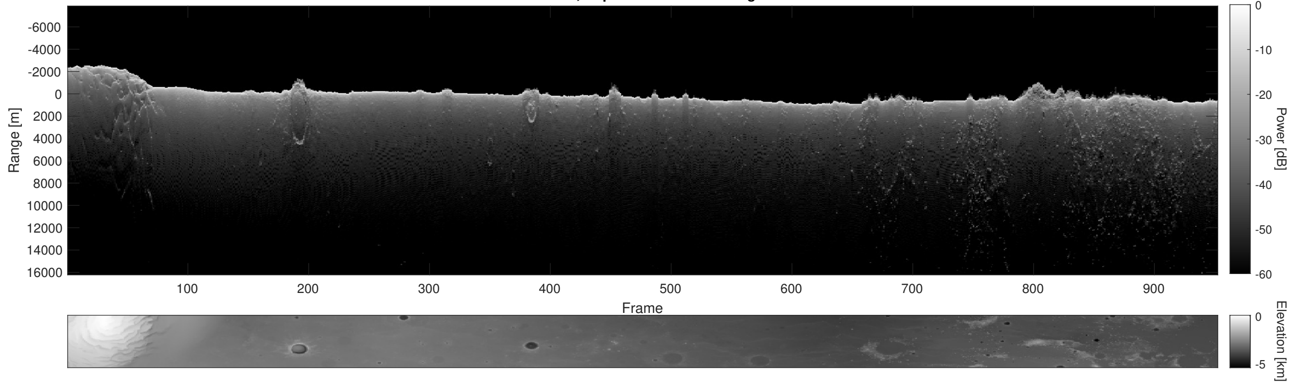
Orbit 11595, Depth-Corrected Cluttergram
