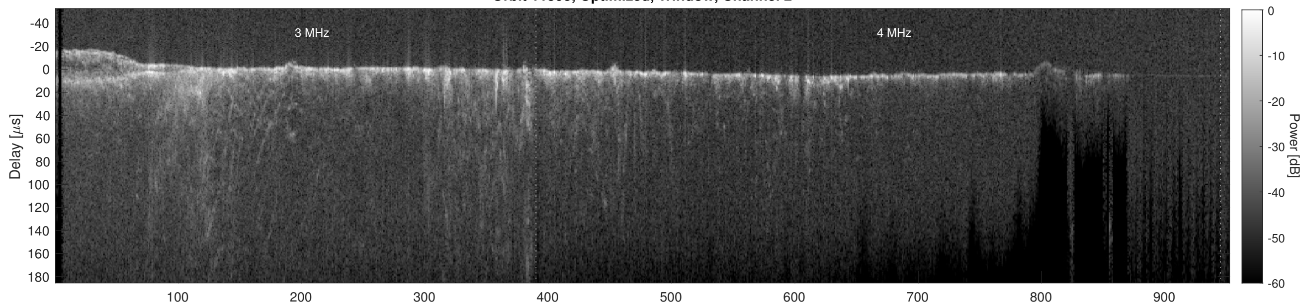
Orbit 11595, Cluttergram
