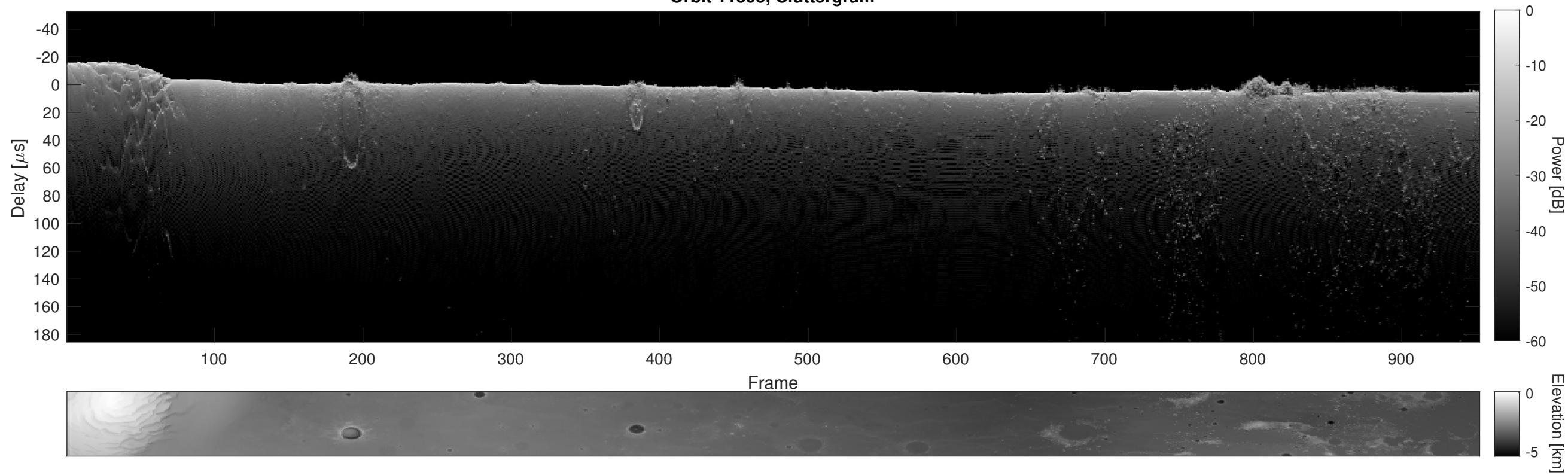
Orbit 11595, Cluttergram
