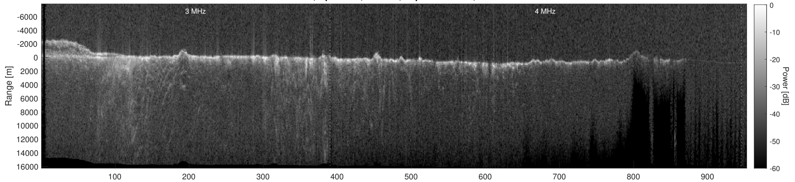
Orbit 11595, Depth-Corrected Cluttergram
