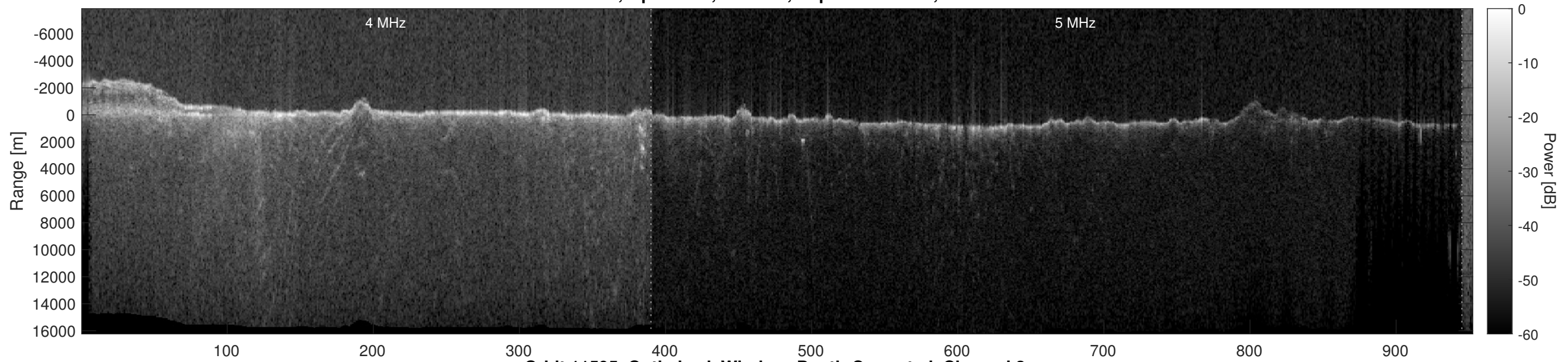
Orbit 11595, Optimized, Window, Depth-Corrected, Channel 2
