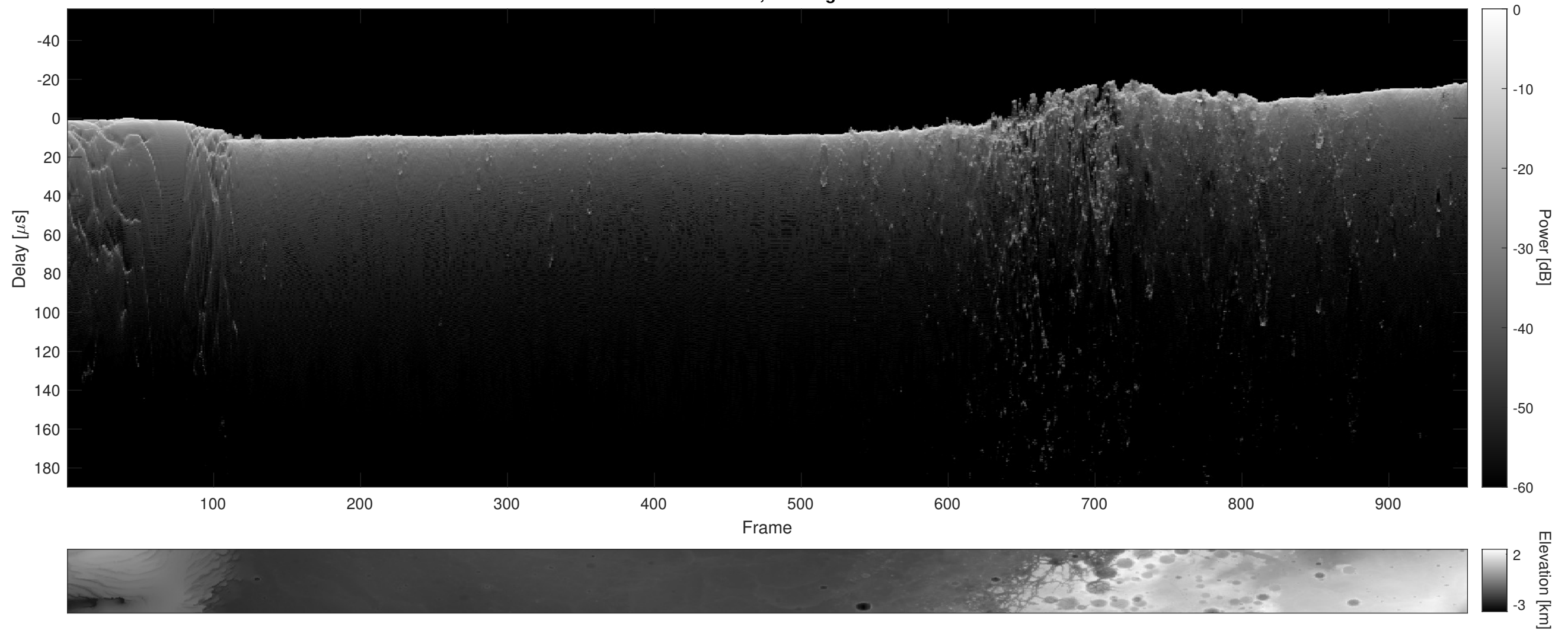
Orbit 11596, Cluttergram
