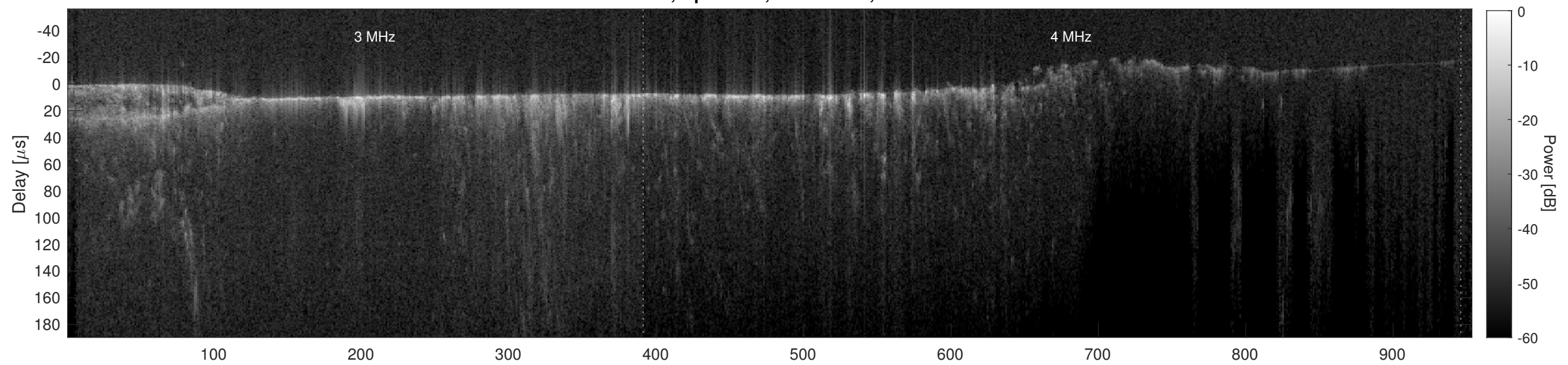
Orbit 11596, Cluttergram
