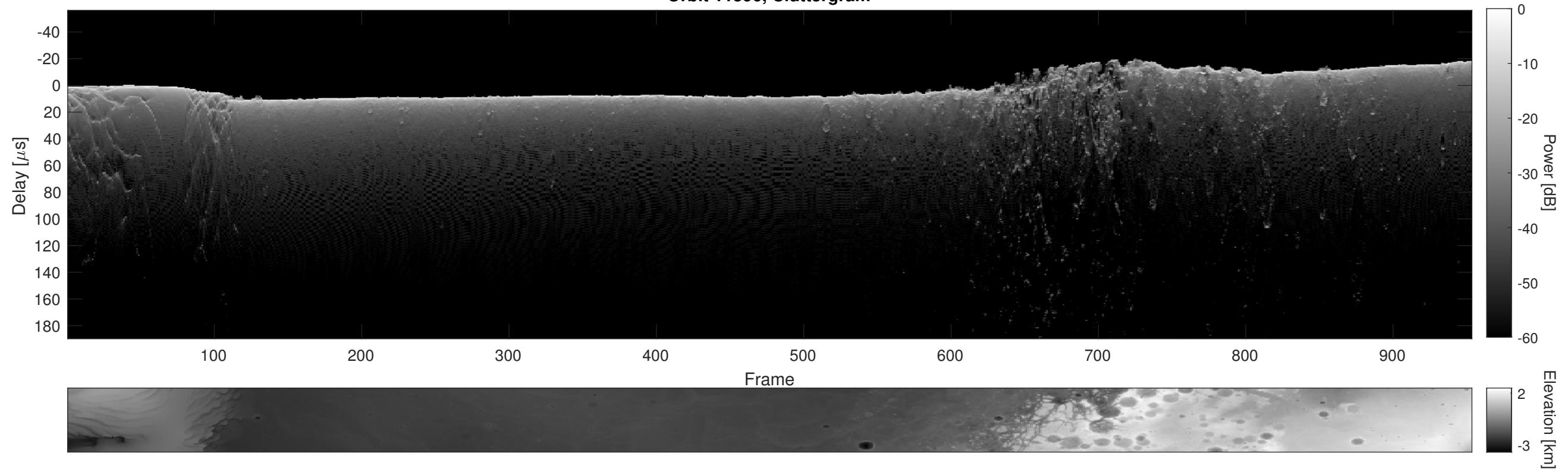
Orbit 11596, Cluttergram
