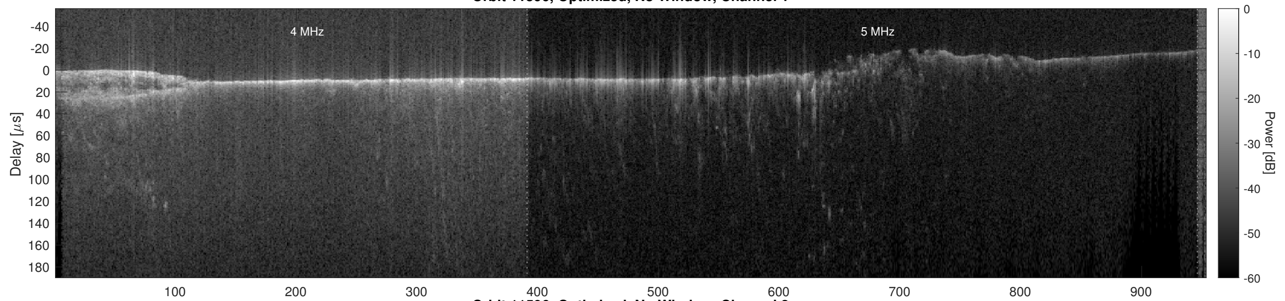
Orbit 11596, Optimized, No Window, Channel 2
