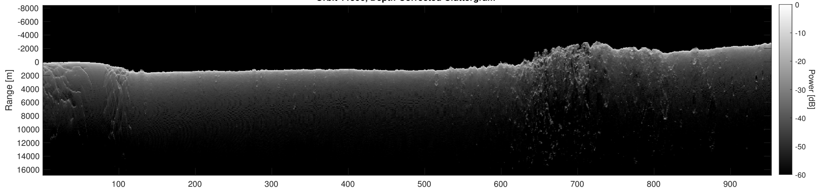
Orbit 11596, Depth-Corrected Cluttergram
