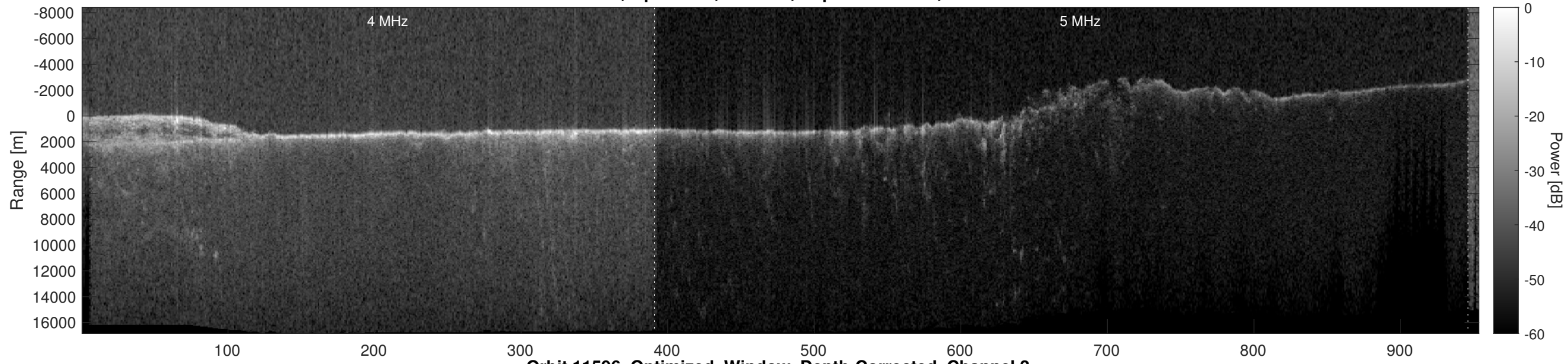
Orbit 11596, Optimized, Window, Depth-Corrected, Channel 2
