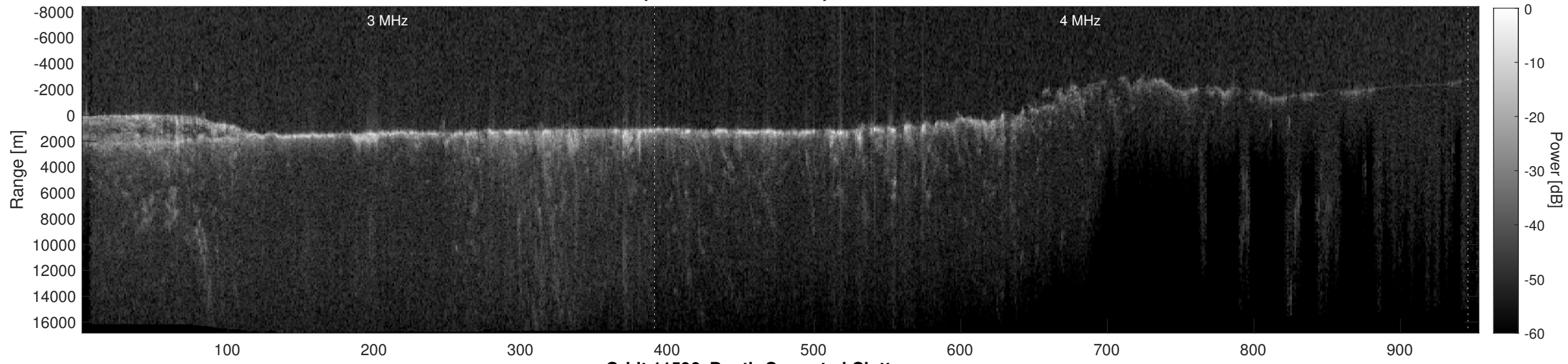
Orbit 11596, Depth-Corrected Cluttergram
