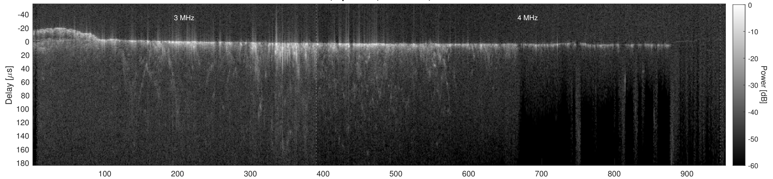
Orbit 11597, Cluttergram
