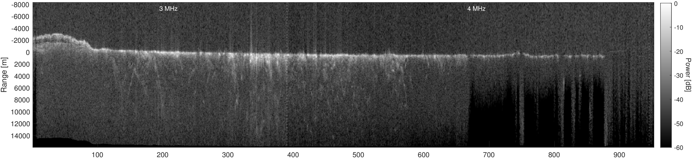
Orbit 11597, Depth-Corrected Cluttergram
