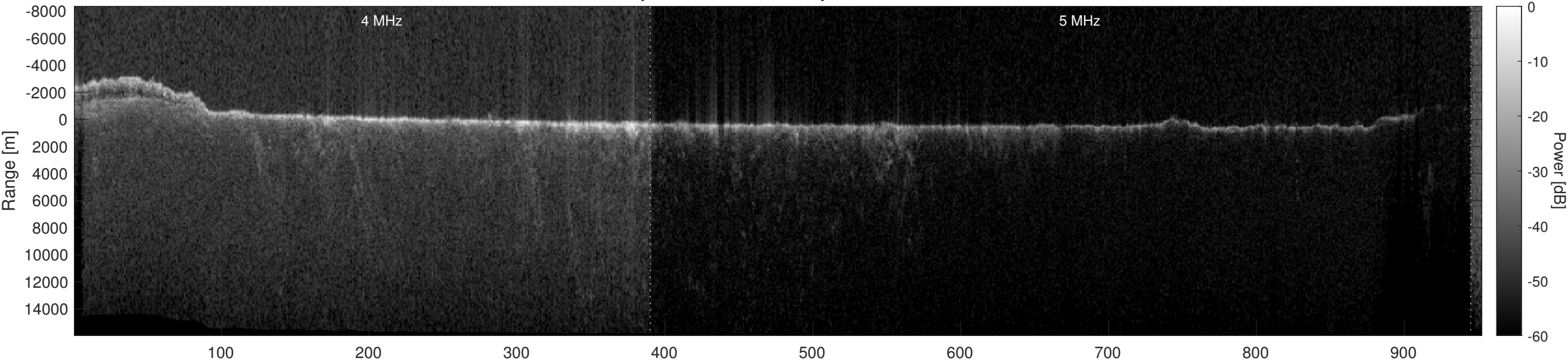
Orbit 11597, Optimized, Window, Depth-Corrected, Channel 2
