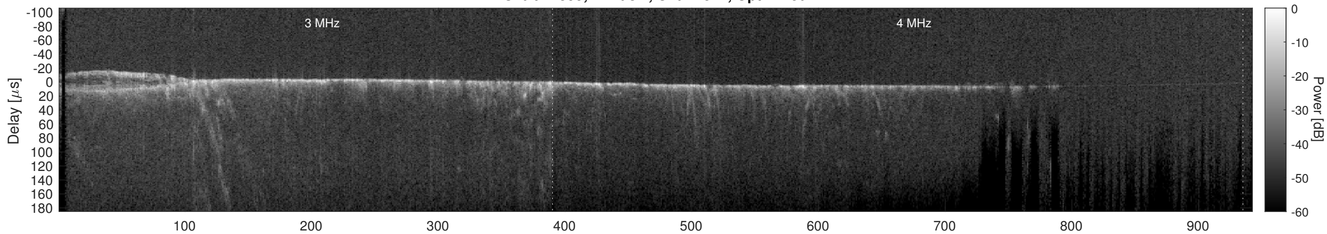
Orbit 11599, Cluttergram
