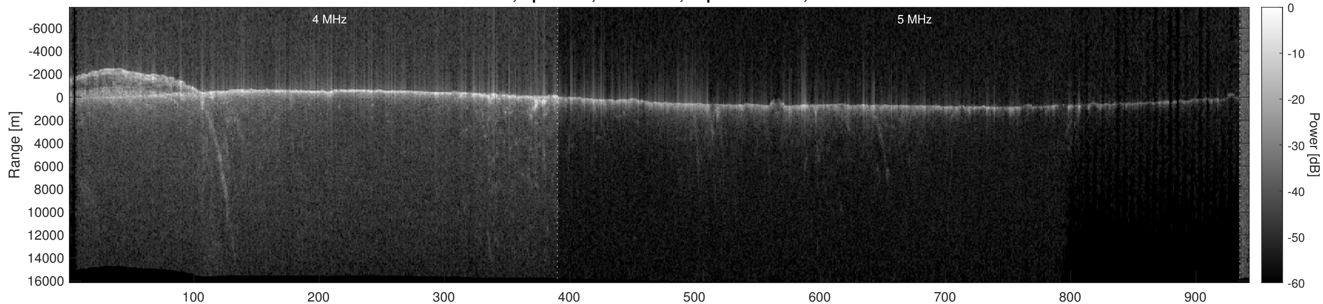
Orbit 11599, Optimized, No Window, Depth-Corrected, Channel 2
