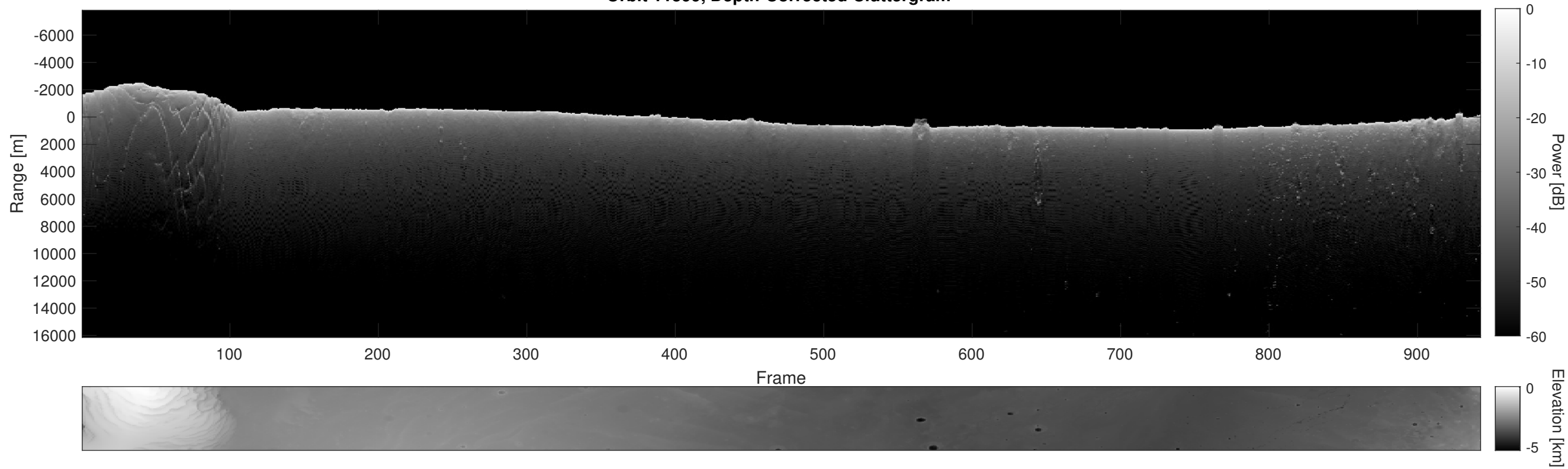
Orbit 11599, Depth-Corrected Cluttergram
