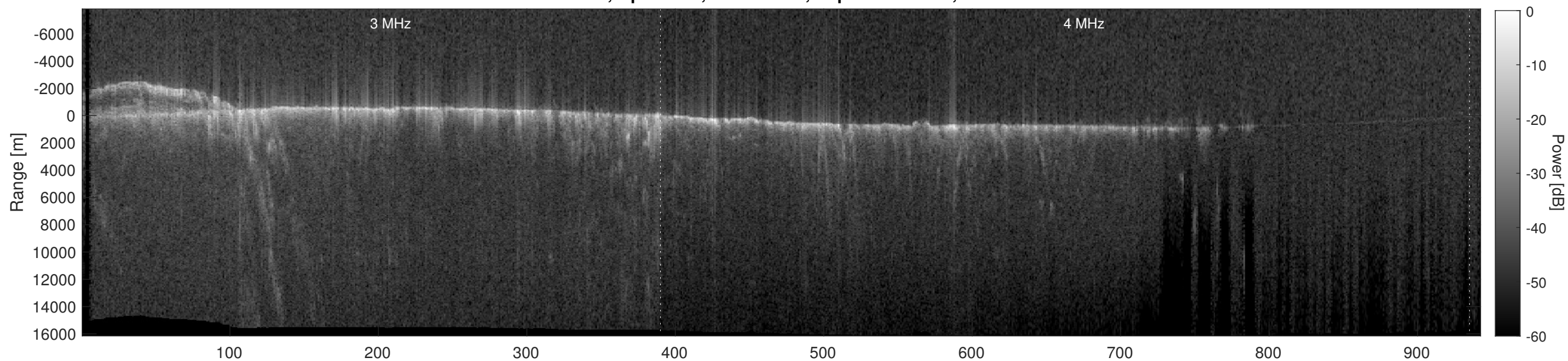
Orbit 11599, Depth-Corrected Cluttergram
