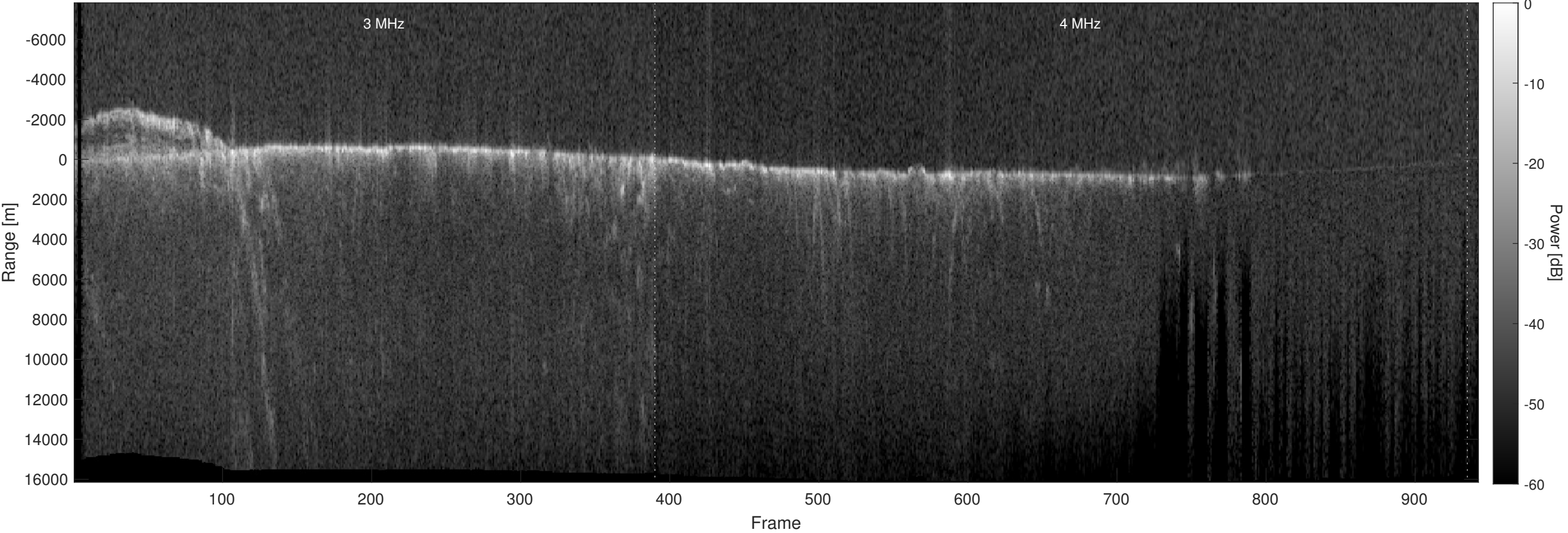
Orbit 11599, Optimized, Window, Depth-Corrected, Channel 2
