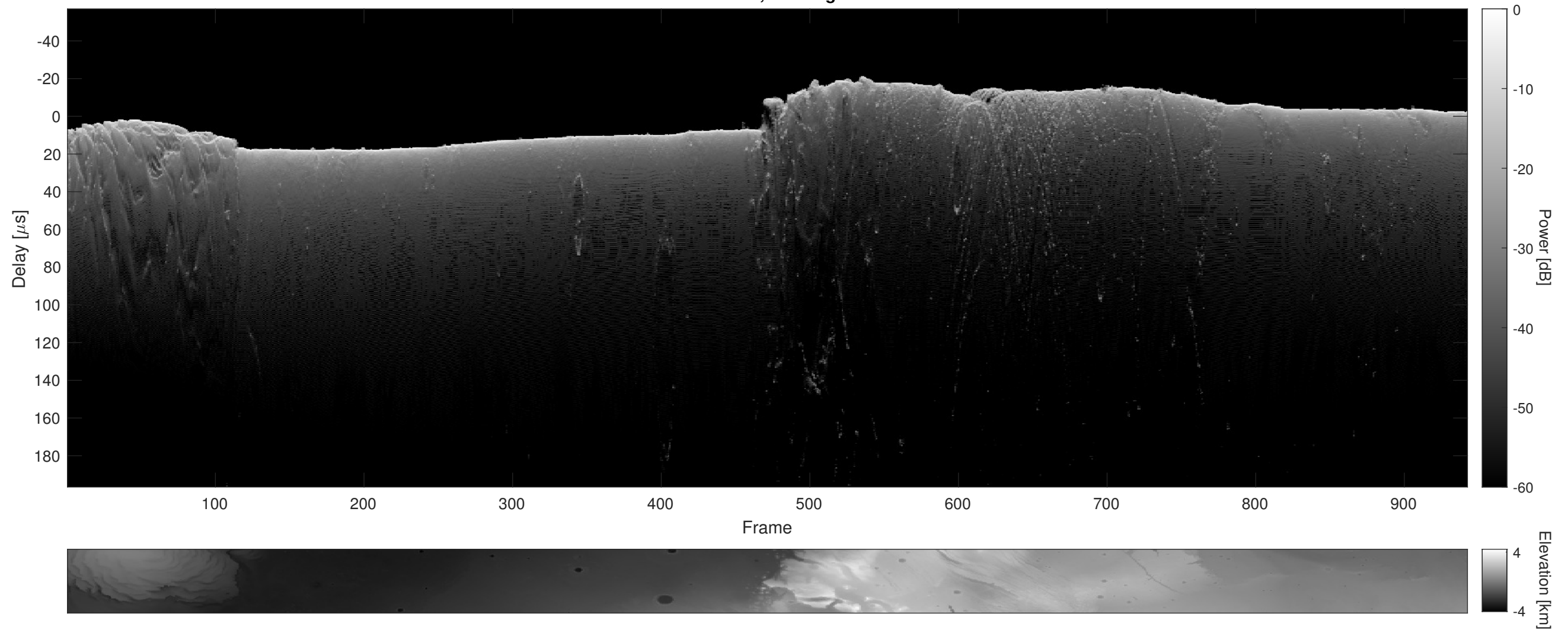
Orbit 11601, Cluttergram
