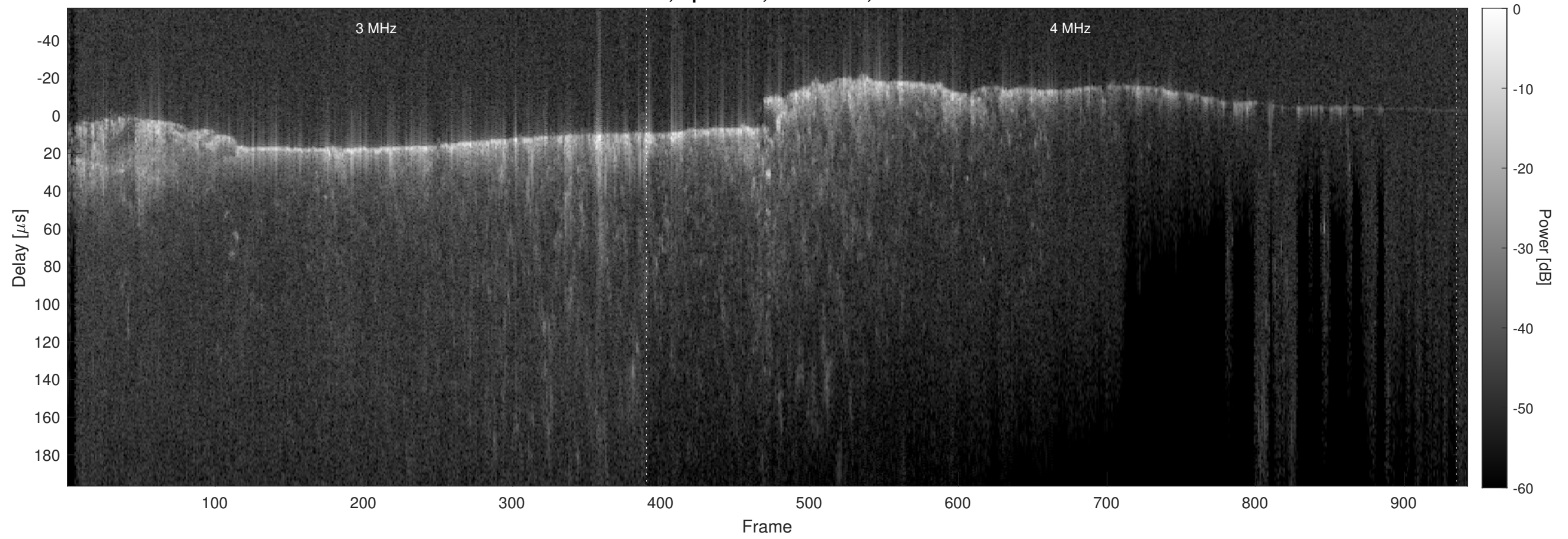
Orbit 11601, Optimized, No Window, Channel 2
