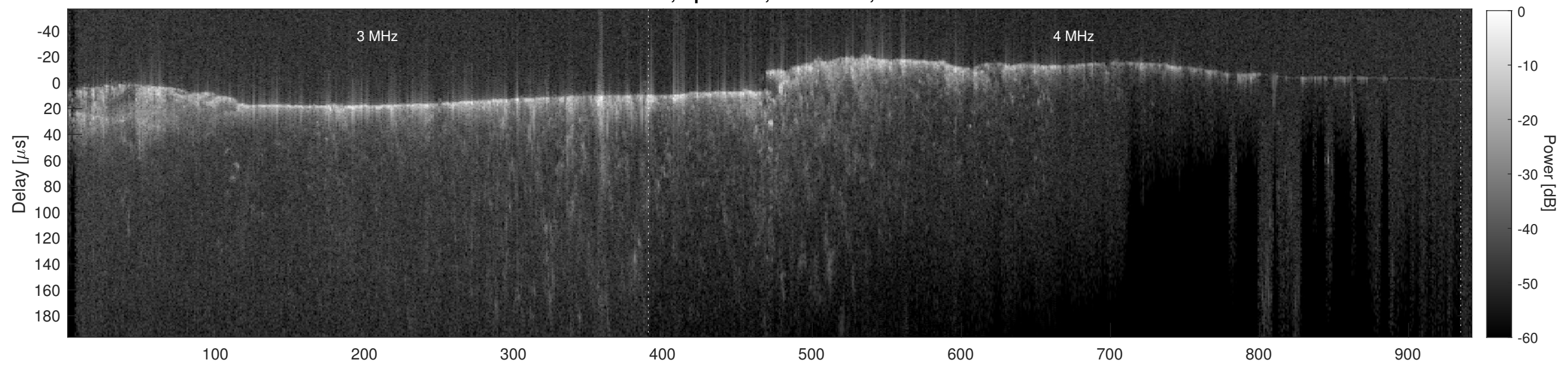
Orbit 11601, Cluttergram
