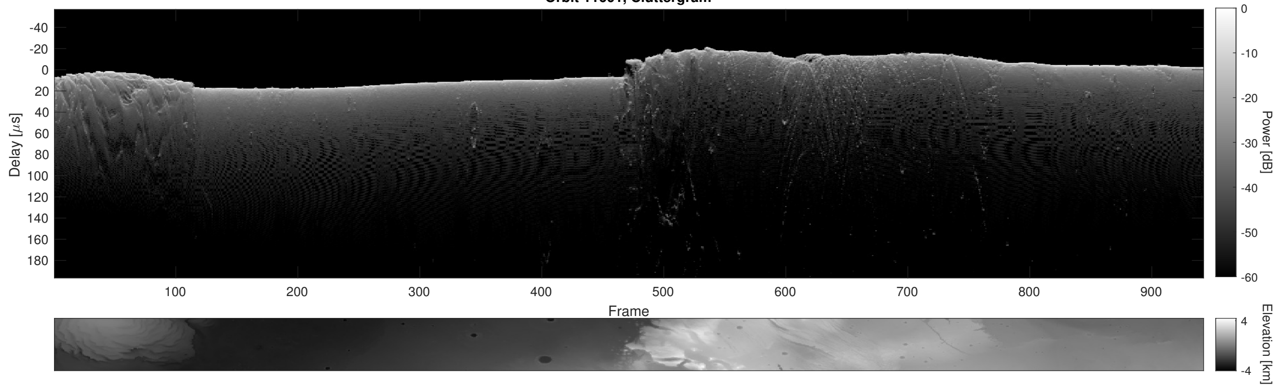
Orbit 11601, Cluttergram
