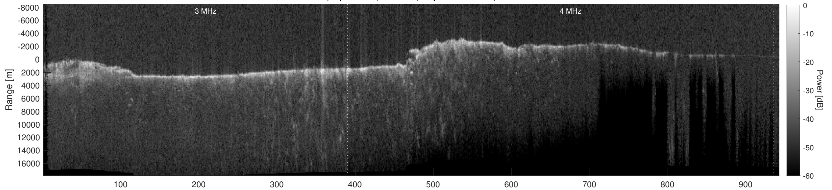
Orbit 11601, Depth-Corrected Cluttergram
