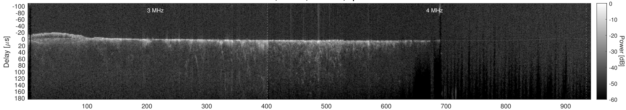
Orbit 11604, Cluttergram
