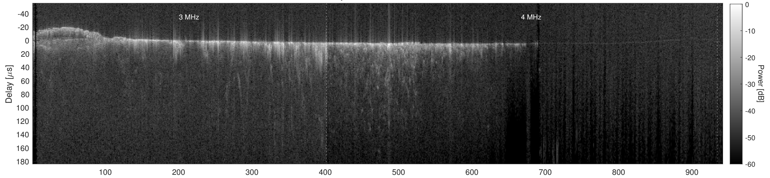
Orbit 11604, Cluttergram
