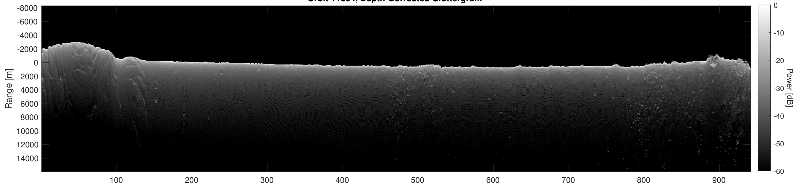
Orbit 11604, Depth-Corrected Cluttergram
