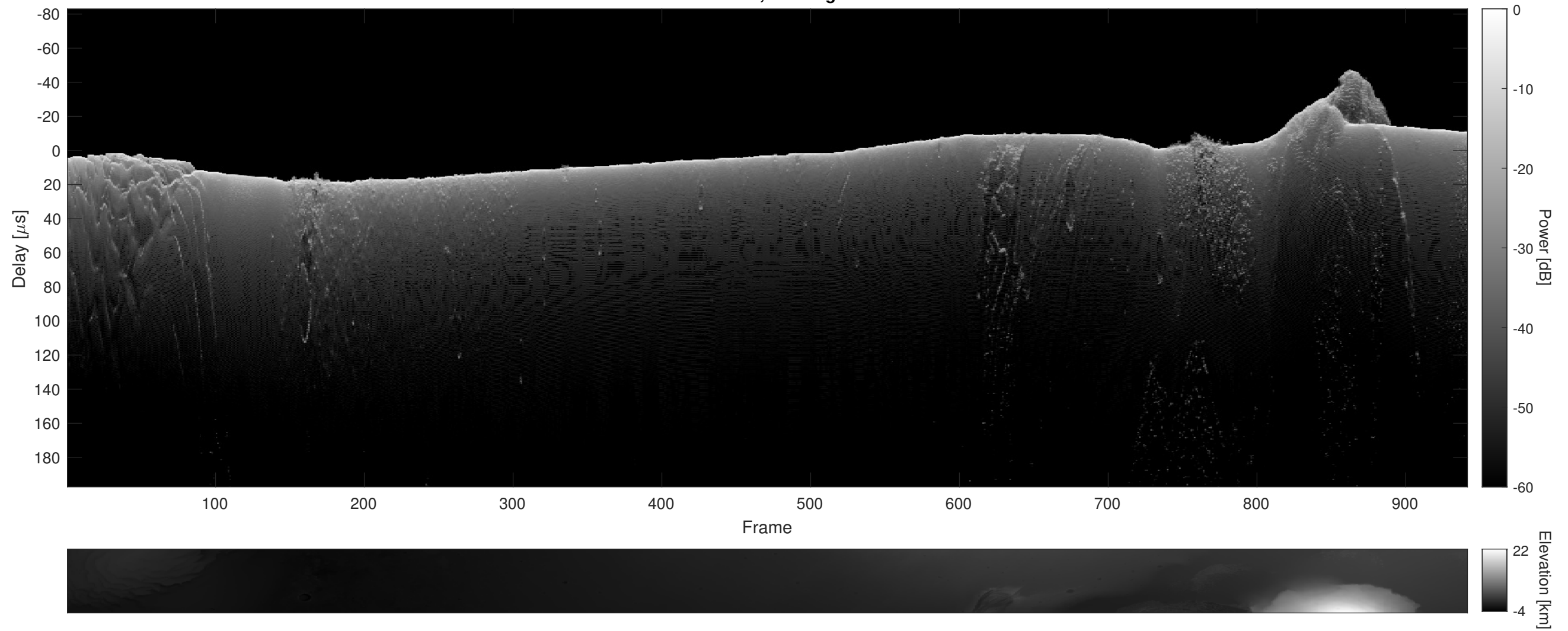
Orbit 11605, Cluttergram
