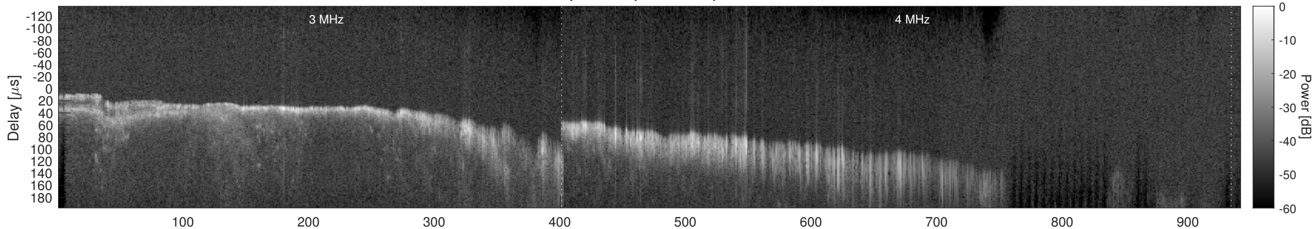
Orbit 11605, Window, Channel 2, Chapman
