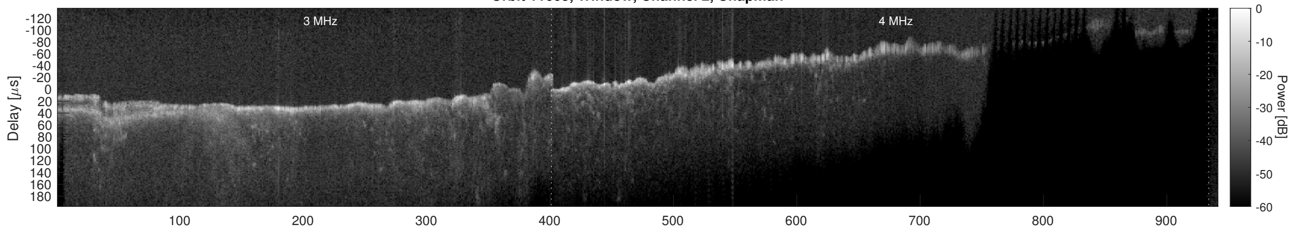
Orbit 11605, Window, Channel 2, Optimized
