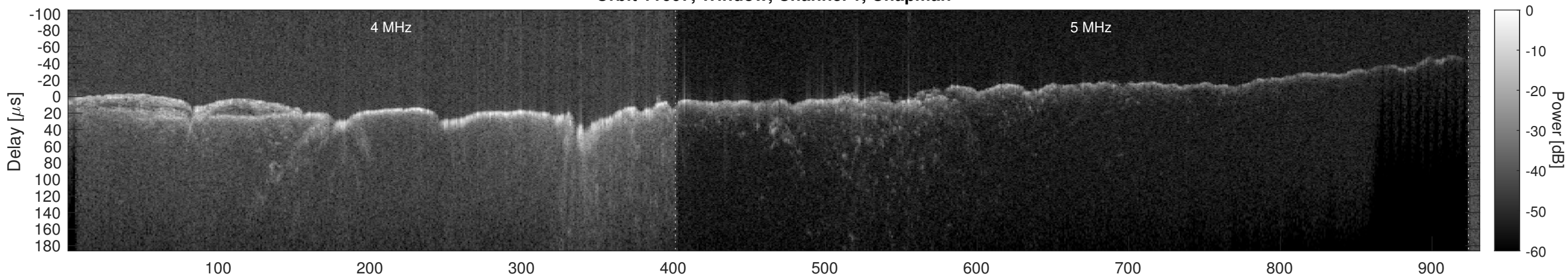
Orbit 11607, Window, Channel 1, Optimized
