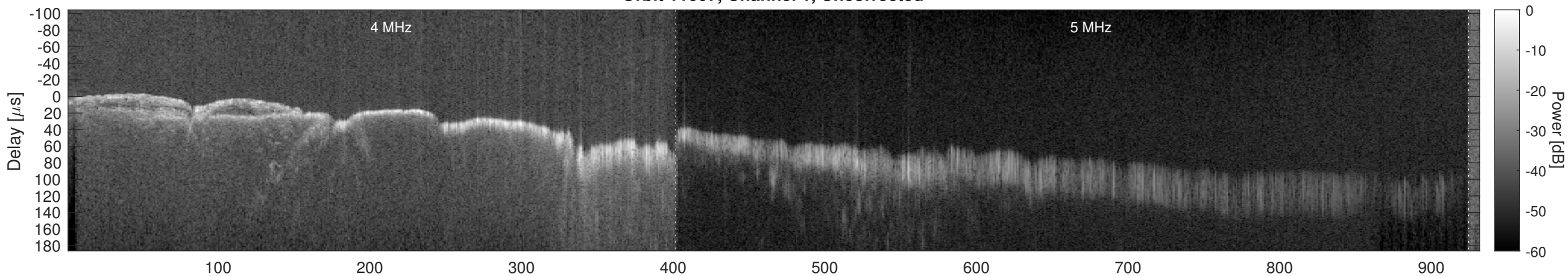
Orbit 11607, Window, Channel 1, Chapman
