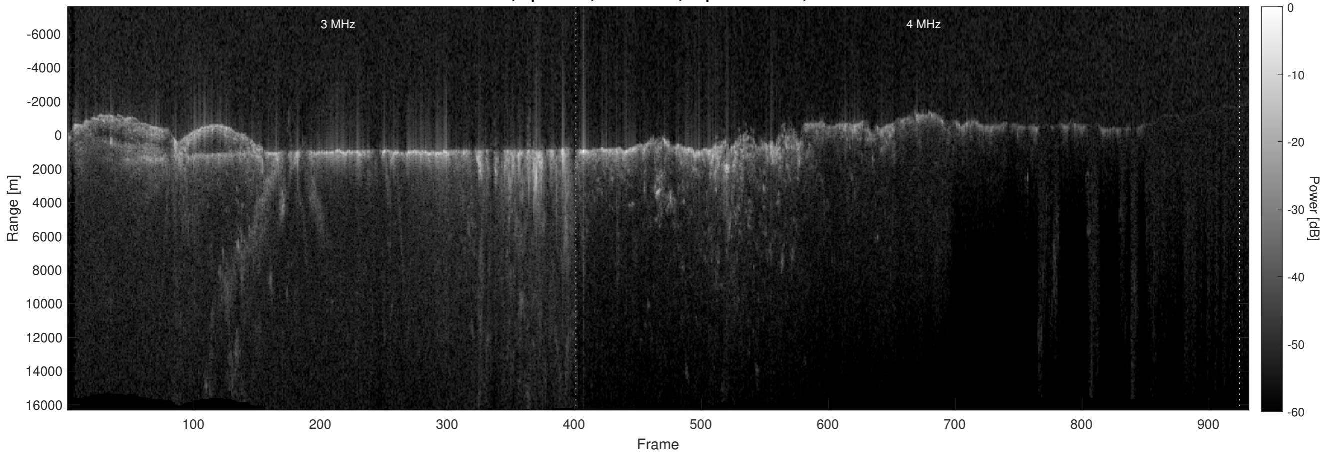
Orbit 11607, Optimized, No Window, Depth-Corrected, Channel 2
