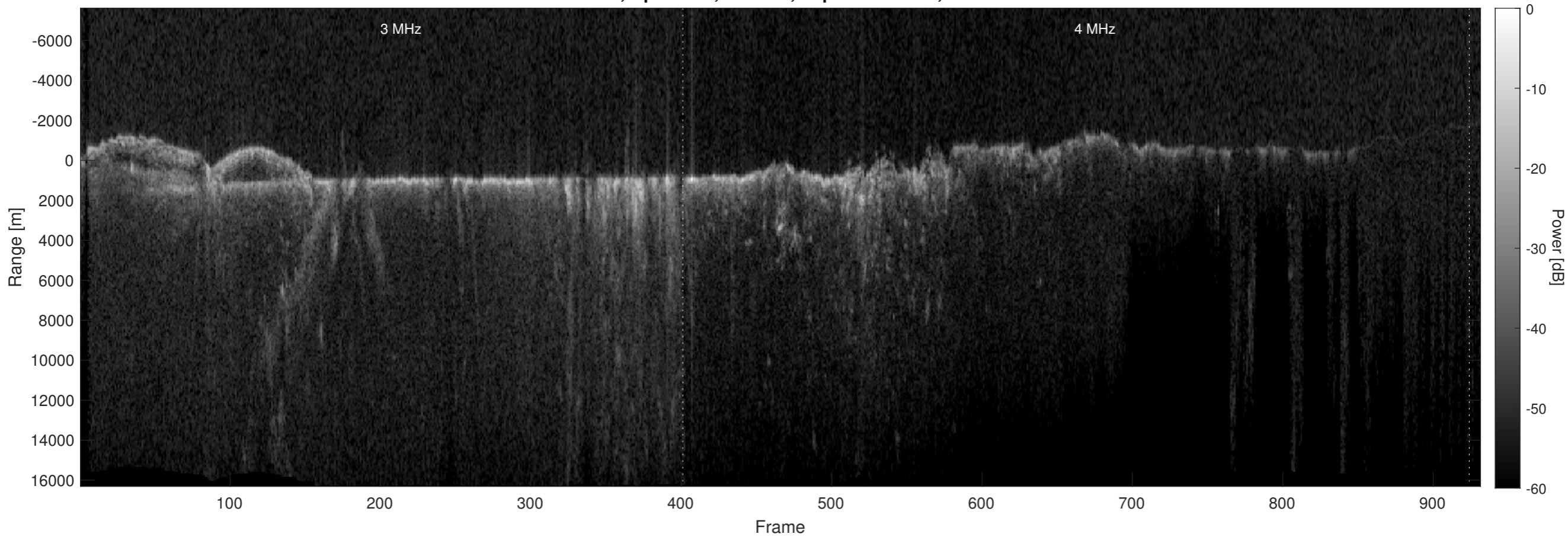
Orbit 11607, Optimized, Window, Depth-Corrected, Channel 2
