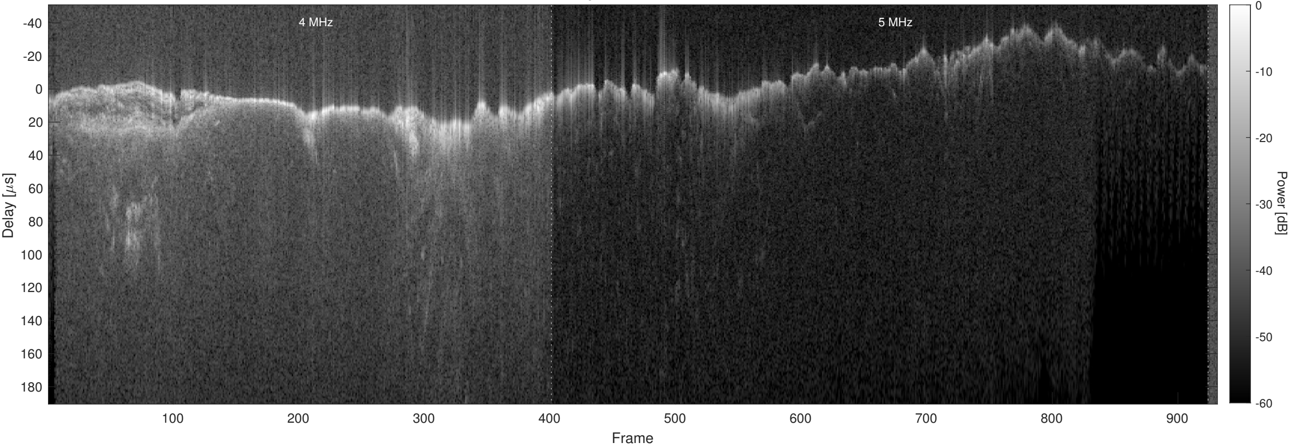
Orbit 11610, Chapman, No Window, Channel 2
