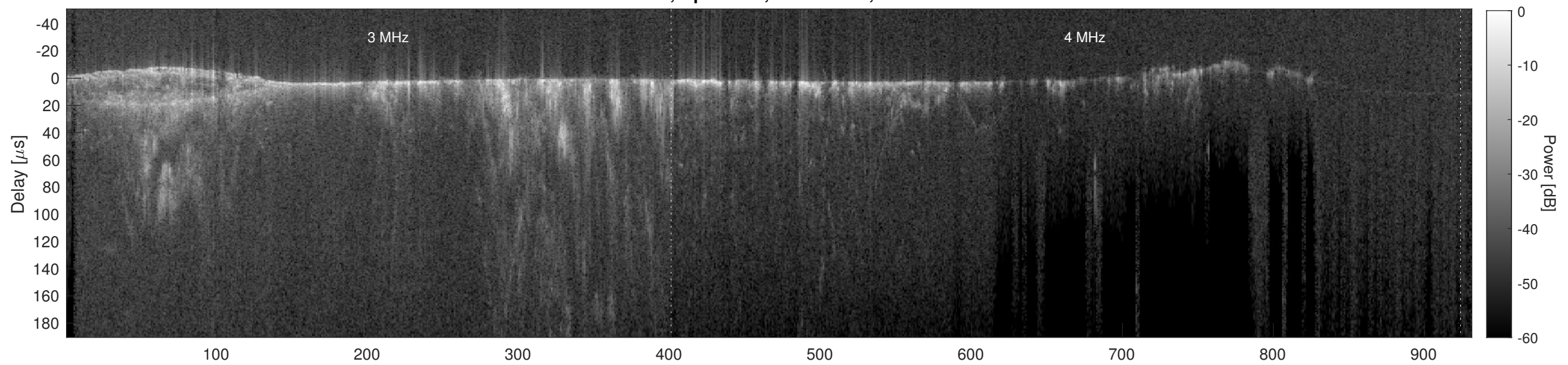
Orbit 11610, Cluttergram
