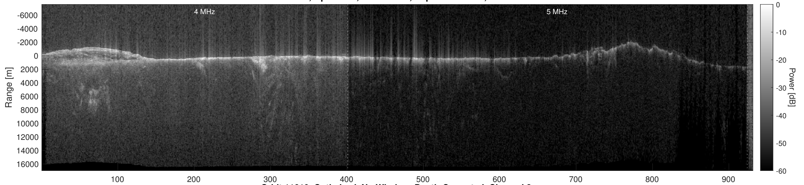
Orbit 11610, Optimized, No Window, Depth-Corrected, Channel 2
