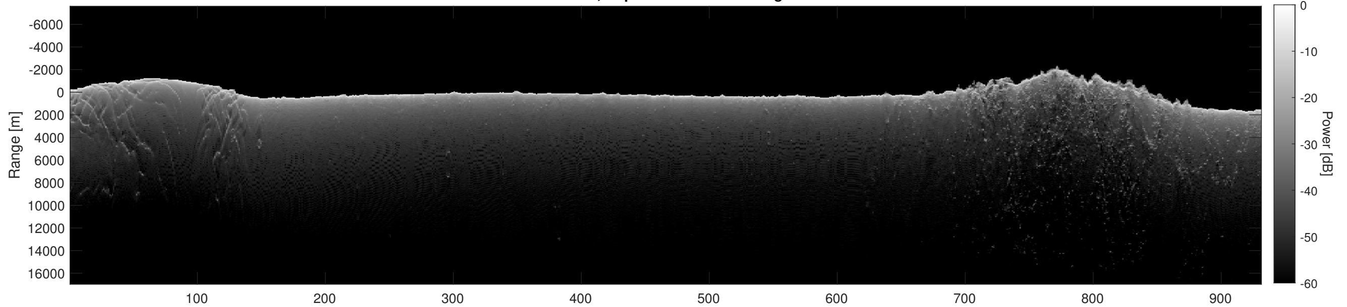
Orbit 11610, Depth-Corrected Cluttergram
