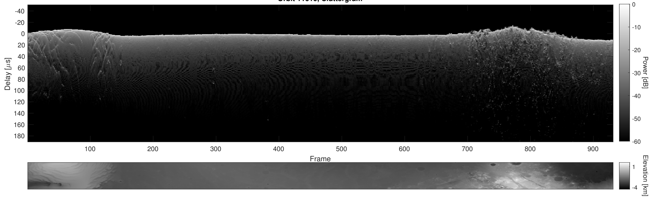
Orbit 11610, Cluttergram
