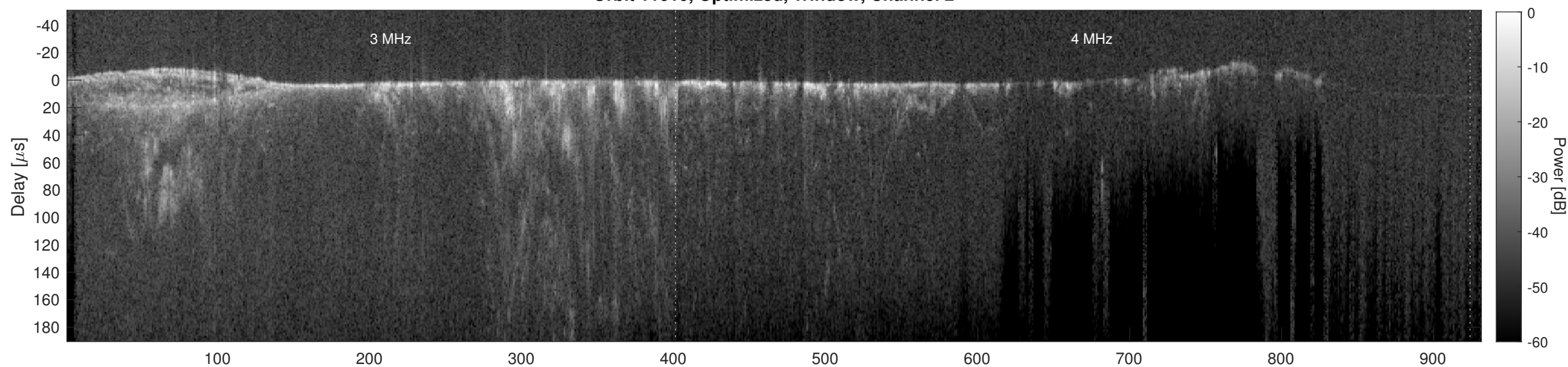
Orbit 11610, Cluttergram
