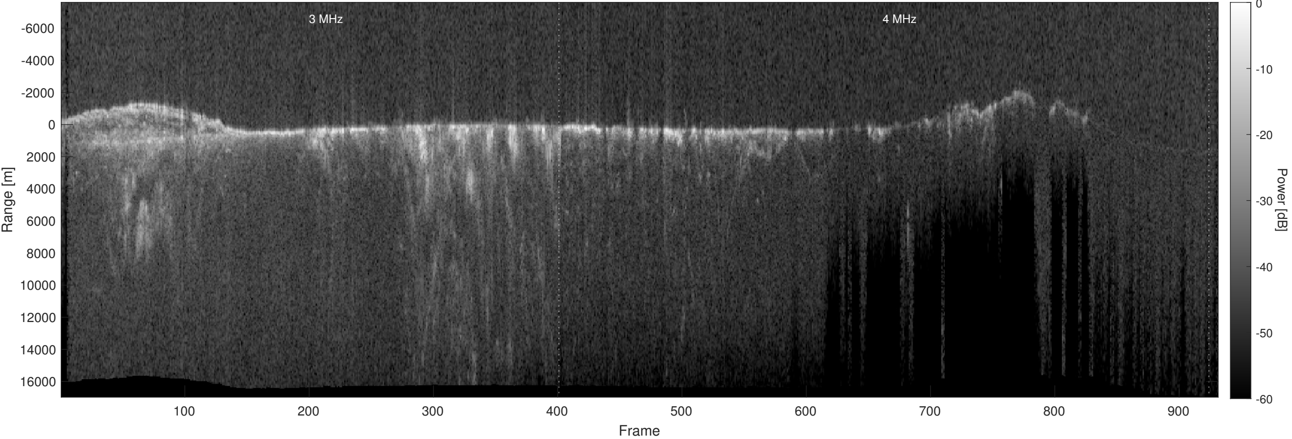
Orbit 11610, Optimized, Window, Depth-Corrected, Channel 2
