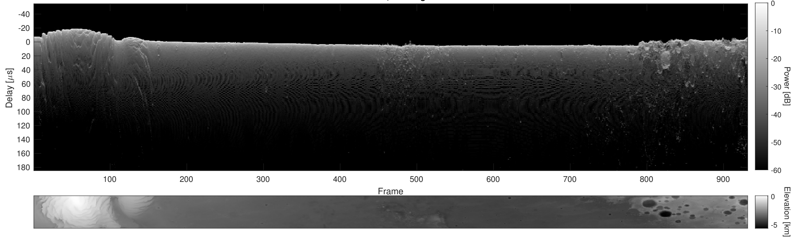
Orbit 11611, Cluttergram
