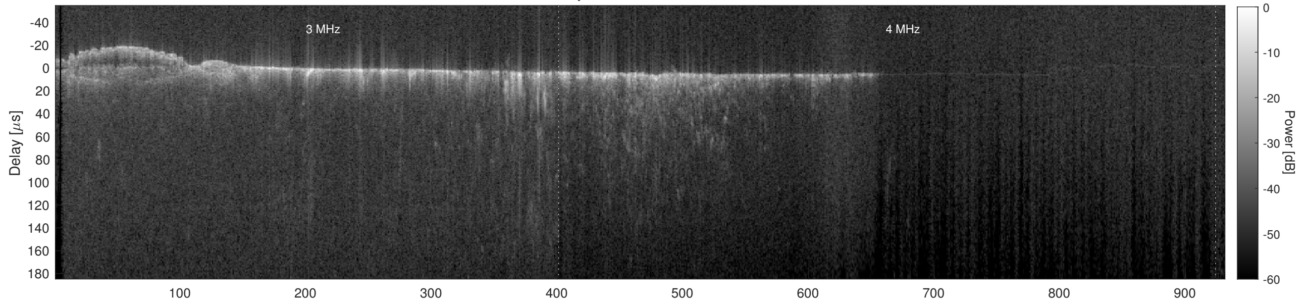
Orbit 11611, Cluttergram
