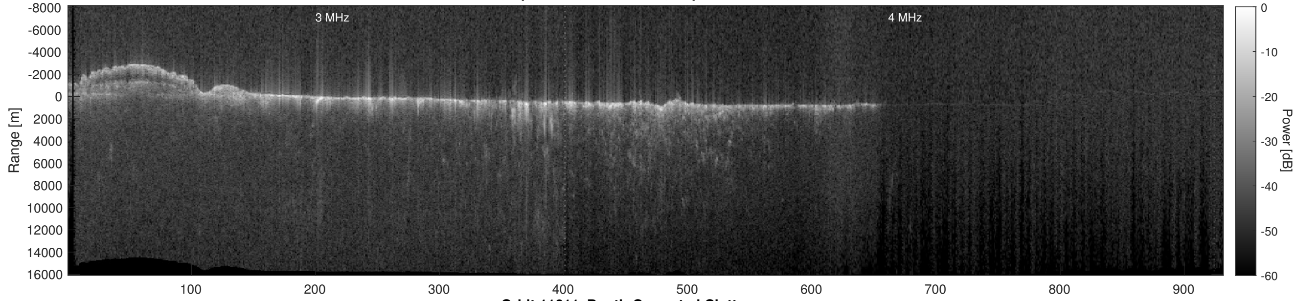
Orbit 11611, Depth-Corrected Cluttergram
