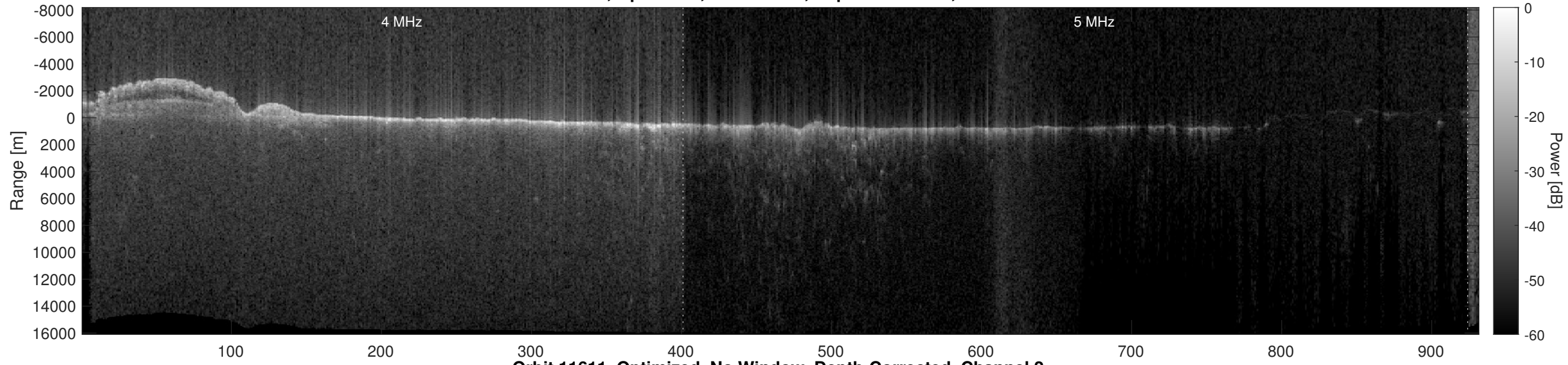
Orbit 11611, Optimized, No Window, Depth-Corrected, Channel 2
