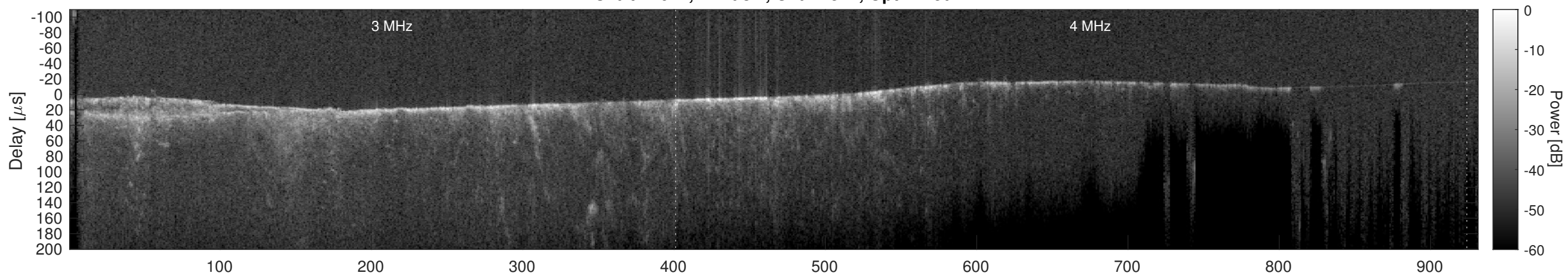
Orbit 11612, Cluttergram
