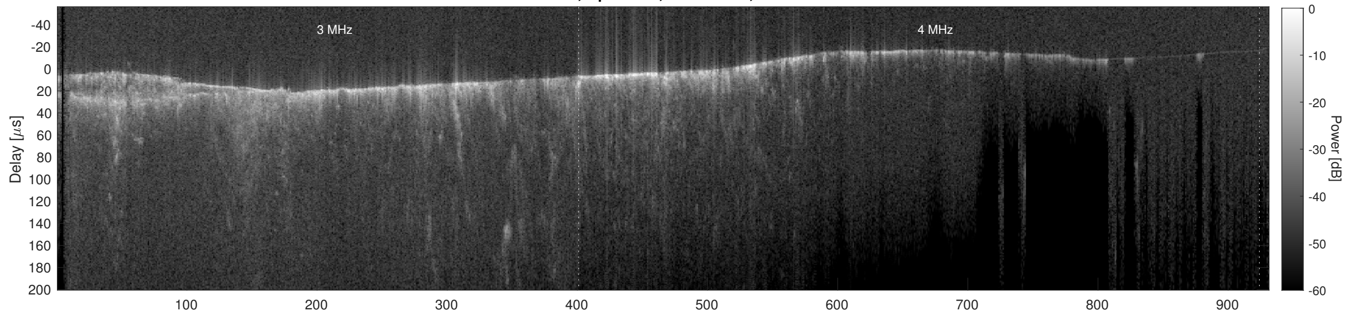
Orbit 11612, Cluttergram
