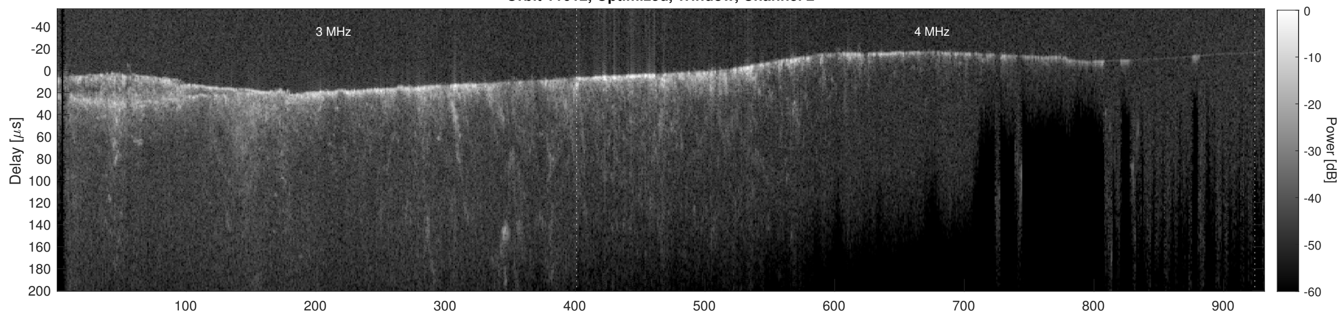
Orbit 11612, Cluttergram
