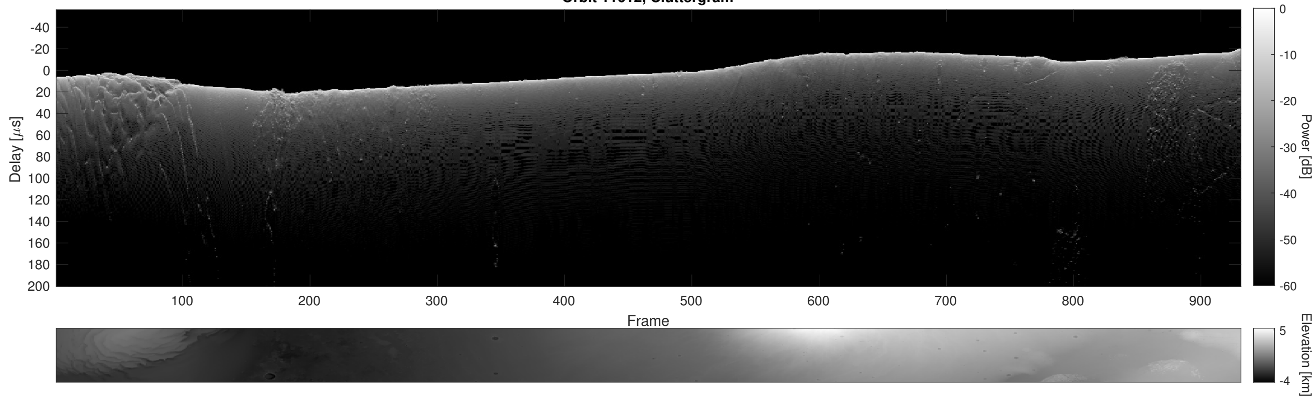
Orbit 11612, Cluttergram
