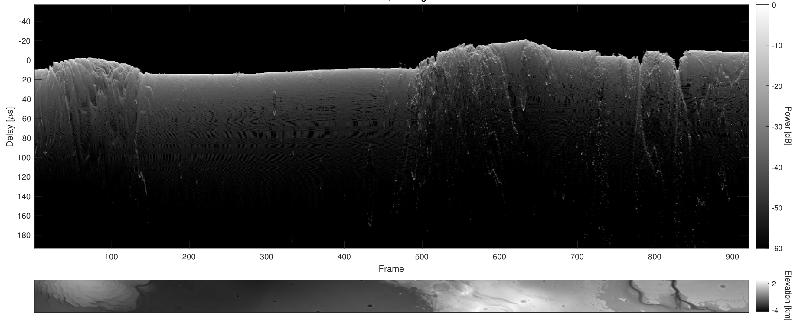
Orbit 11615, Cluttergram
