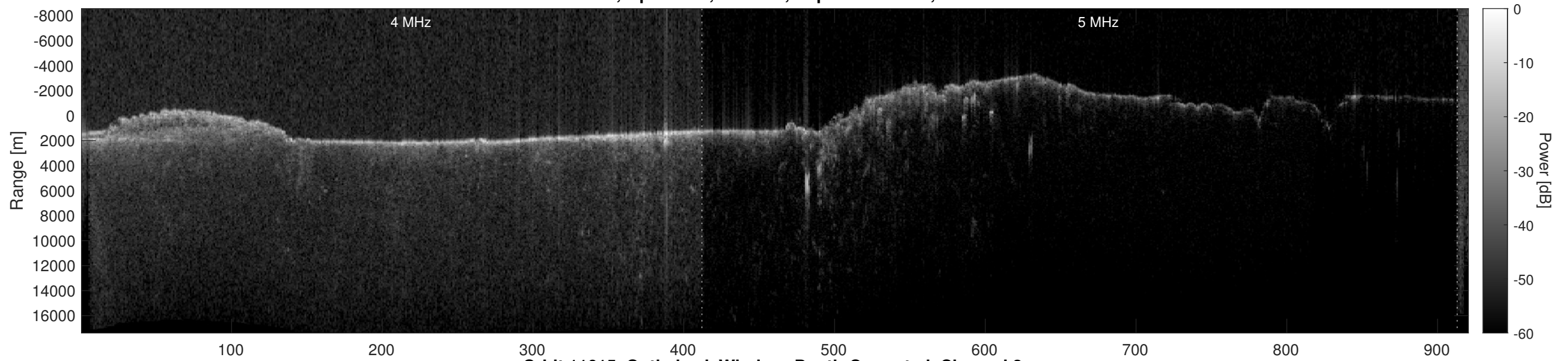
Orbit 11615, Optimized, Window, Depth-Corrected, Channel 2
