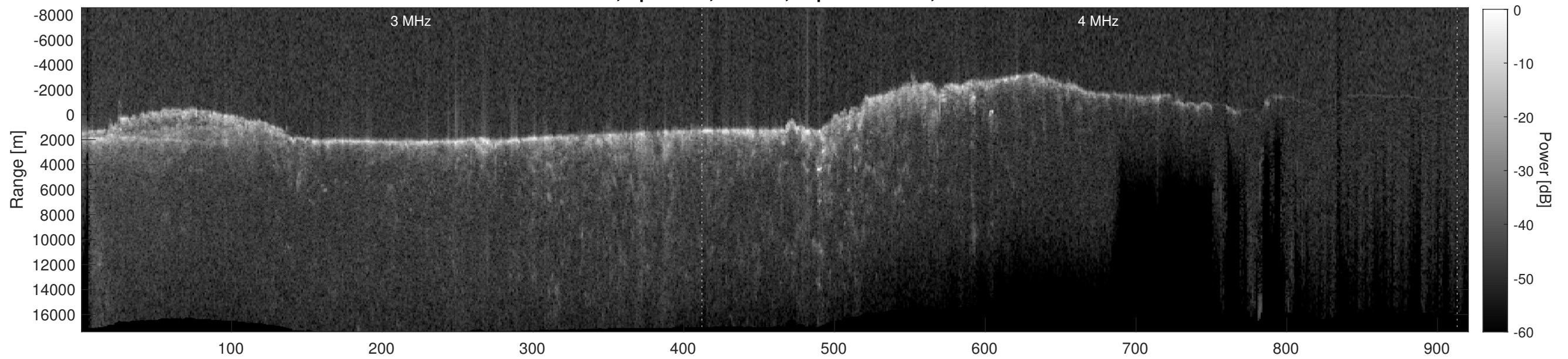
Orbit 11615, Depth-Corrected Cluttergram
