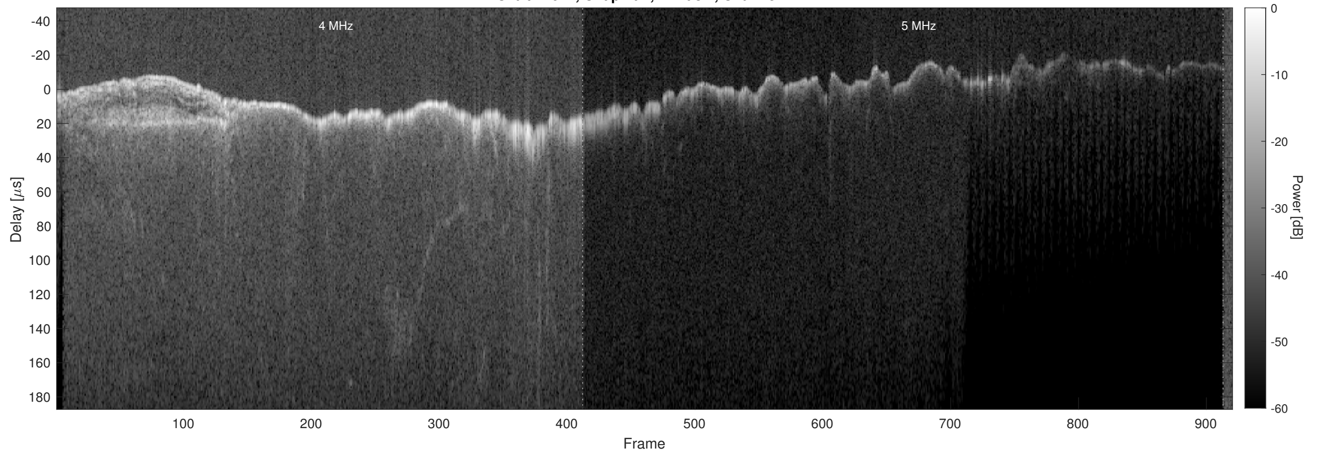
Orbit 11617, Chapman, Window, Channel 2
