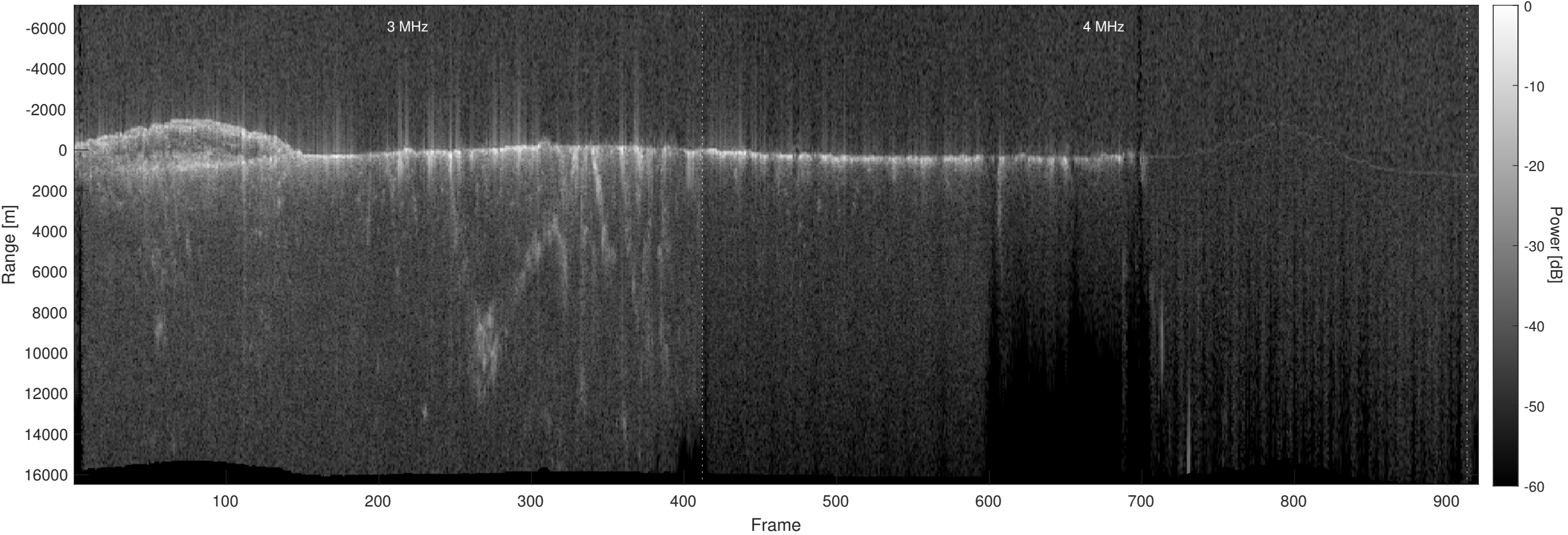
Orbit 11617, Optimized, No Window, Depth-Corrected, Channel 2
