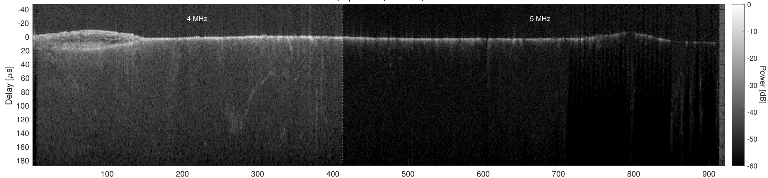
Orbit 11617, Optimized, Window, Channel 2
