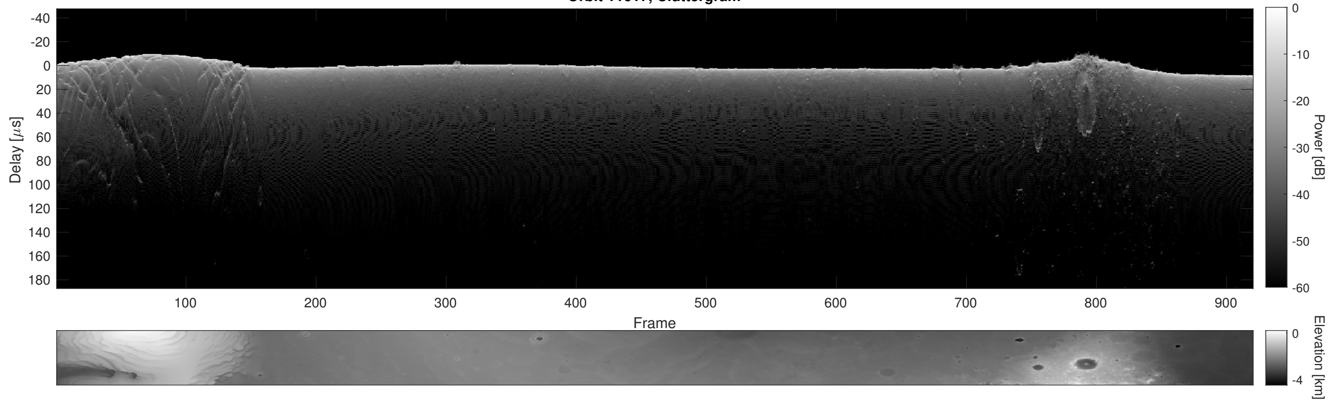
Orbit 11617, Cluttergram
