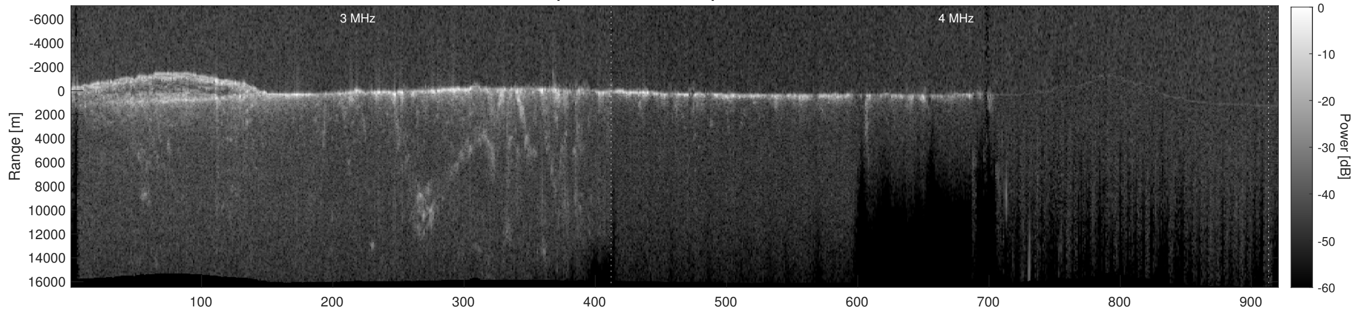
Orbit 11617, Depth-Corrected Cluttergram
