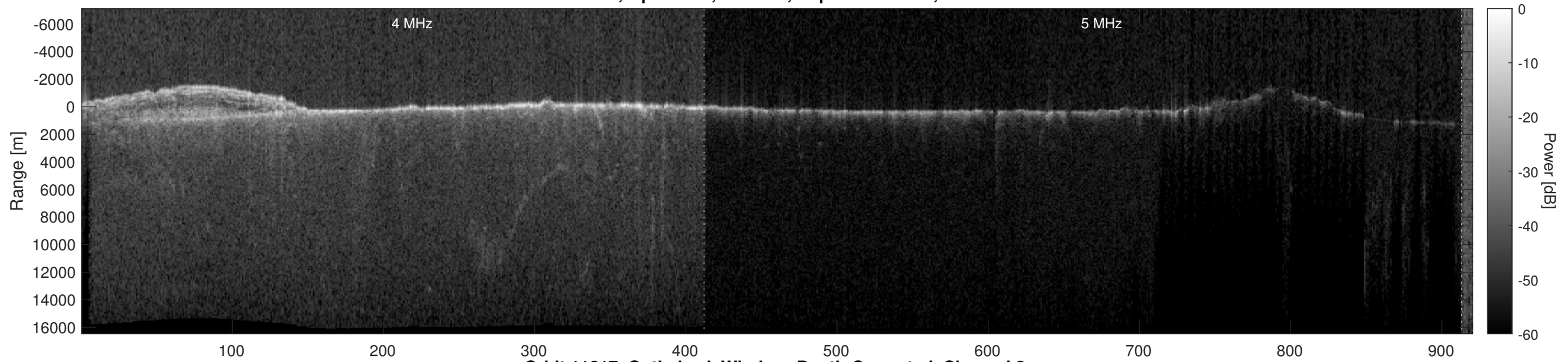
Orbit 11617, Optimized, Window, Depth-Corrected, Channel 2
