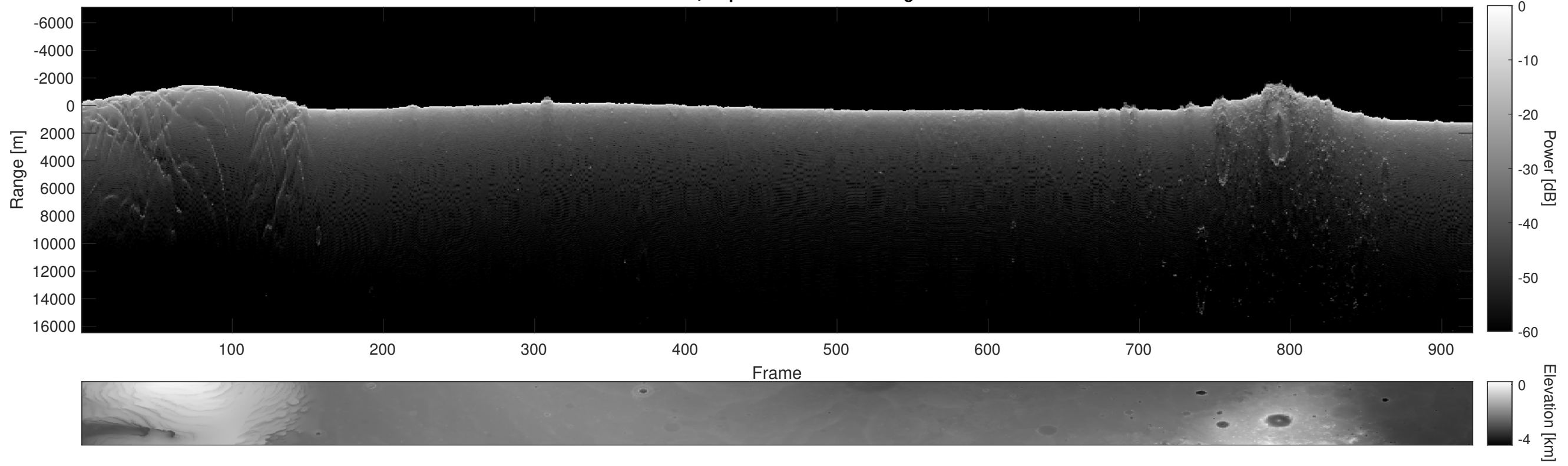
Orbit 11617, Depth-Corrected Cluttergram
