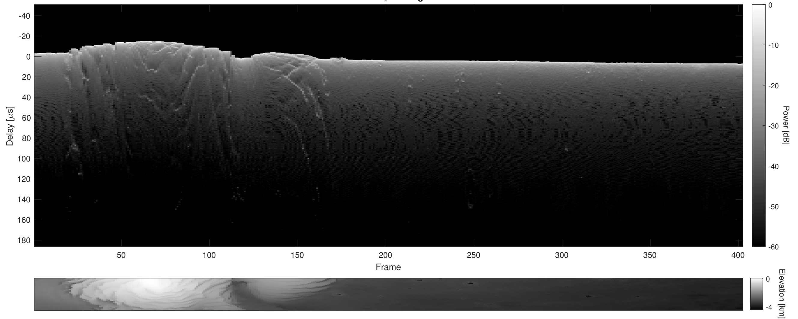
Orbit 11618, Cluttergram
