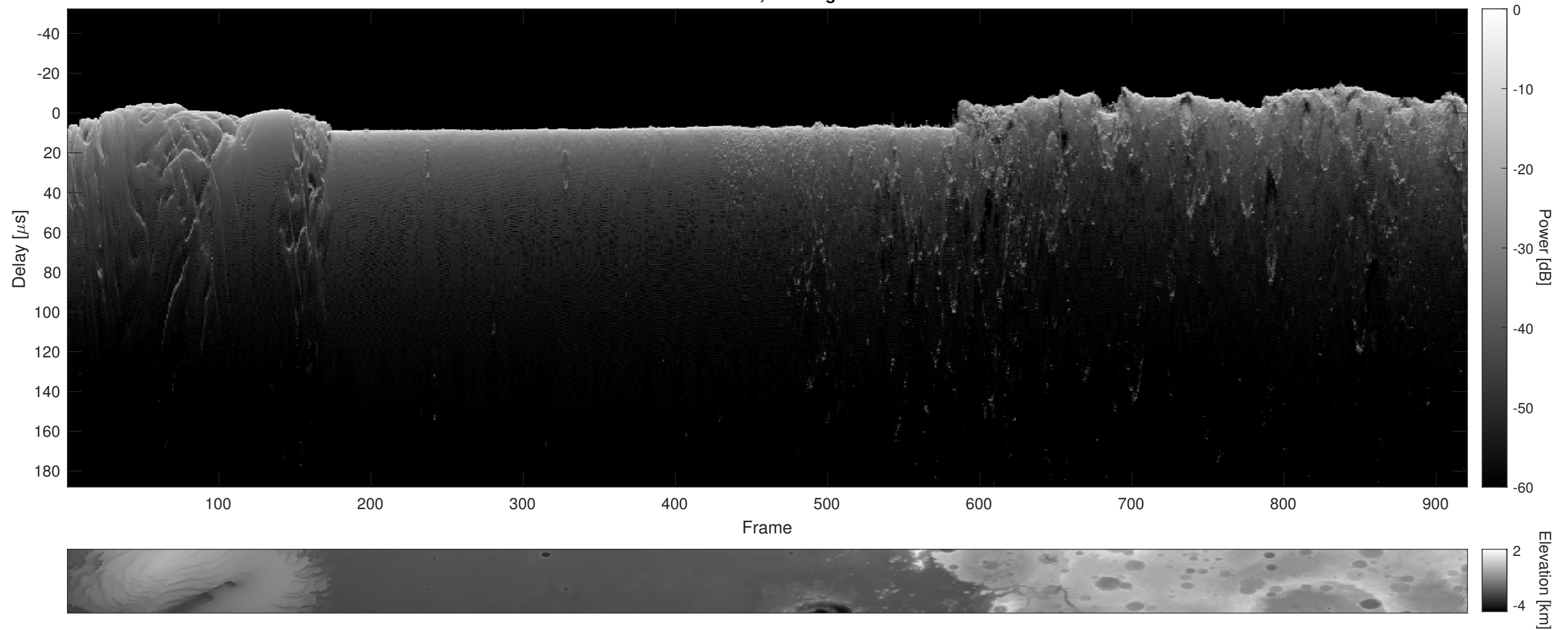
Orbit 11621, Cluttergram
