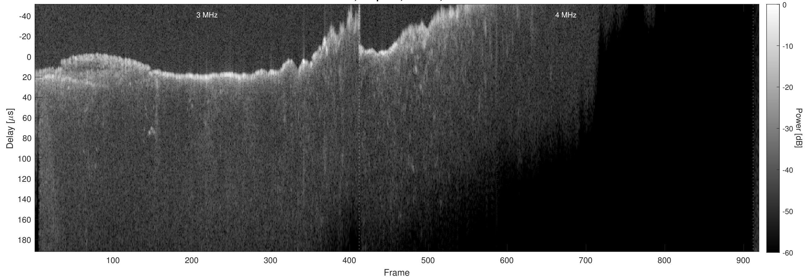
Orbit 11622, Chapman, Window, Channel 2
