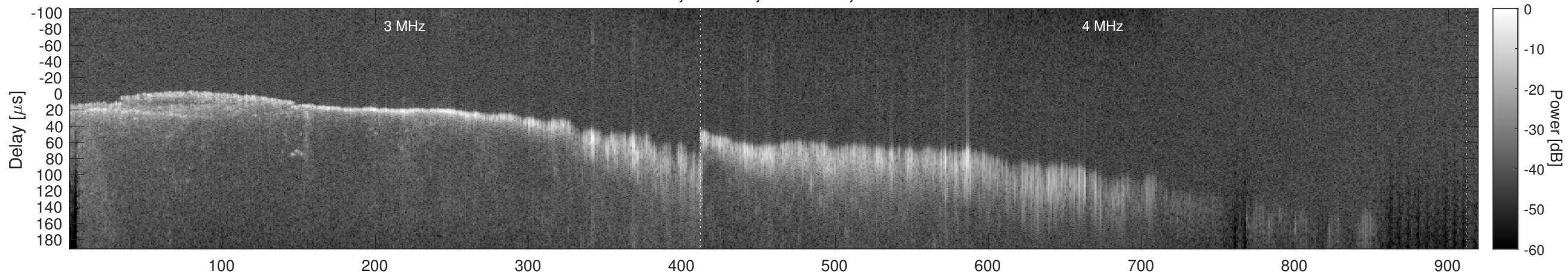
Orbit 11622, Window, Channel 2, Chapman
